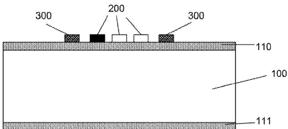
FIG. 3. Deposition of heater and temperature sensor.
