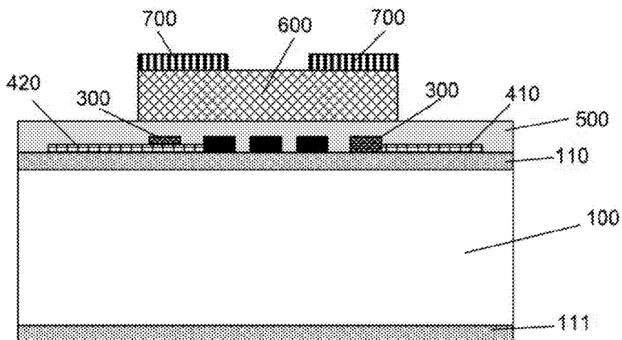
FIG 7. Form electrodes.
