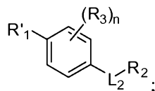
Formula (IIA).
