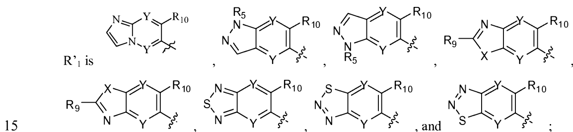
Formula (II);
