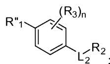
Formula (IIIA).
