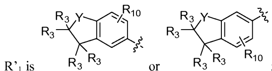
Formula (VII);
