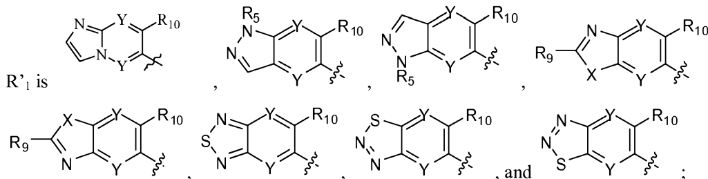
Formula (II);
