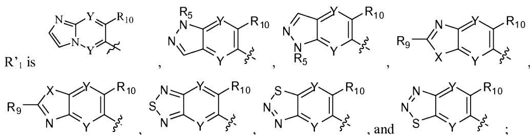
Formula (II);
