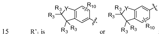
Formula (VII);
