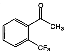
[Chem. 4]
