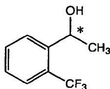
[Chem. 7]
