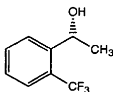
[Chem. 9]
