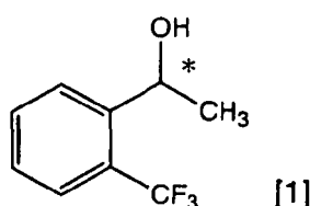
[Chem. 1]
