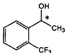
[Chem. 8]
