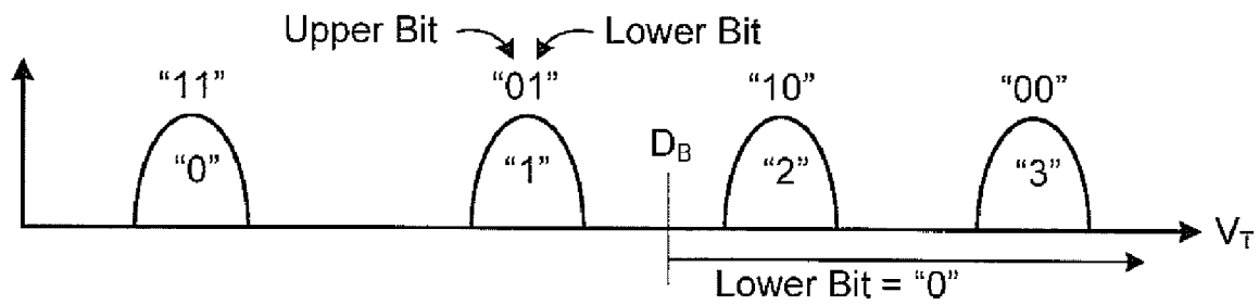
Lower Page Read (2-bit Code)
