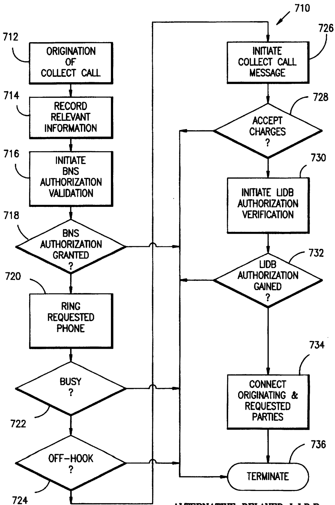
ALTERNATIVE DELAYED L.I.D.B. COLLECT CALL SCHEME
