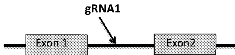
HPRT Genomic Region
