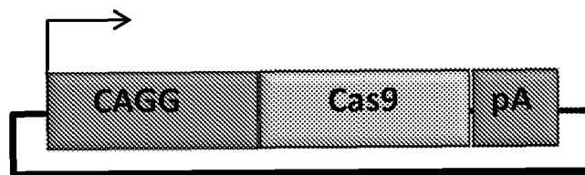
Cas9 Nuclease (10 kb)
