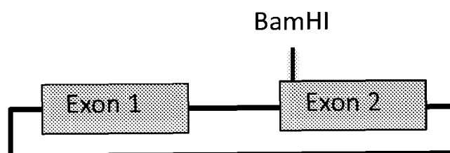
HPRT 'Target' Vector (3.6 kb)
