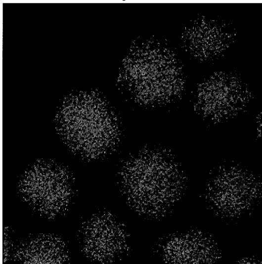
Pd 0.9 -Ru 0.1 alloy fine particles Pd-L EDX map
