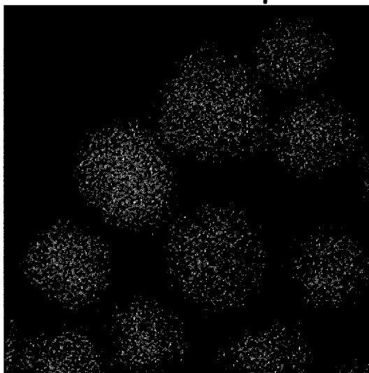
Pd 0.9 -Ru 0.1 alloy fine particles Ru-L + Pd-L EDX map
