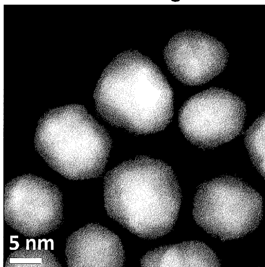
Pd 0.9 -Ru 0.1 alloy fine particles HAADF-STEM image
