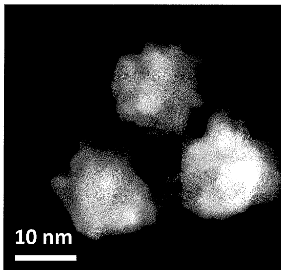
Pd 0.3 -Ru 0.7 alloy fine particles HAADF-STEM image
