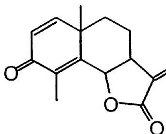
3-KETO-EUDISM-1(2), 4(5), 11(13)-TRIENE-6-12-OLID 18
