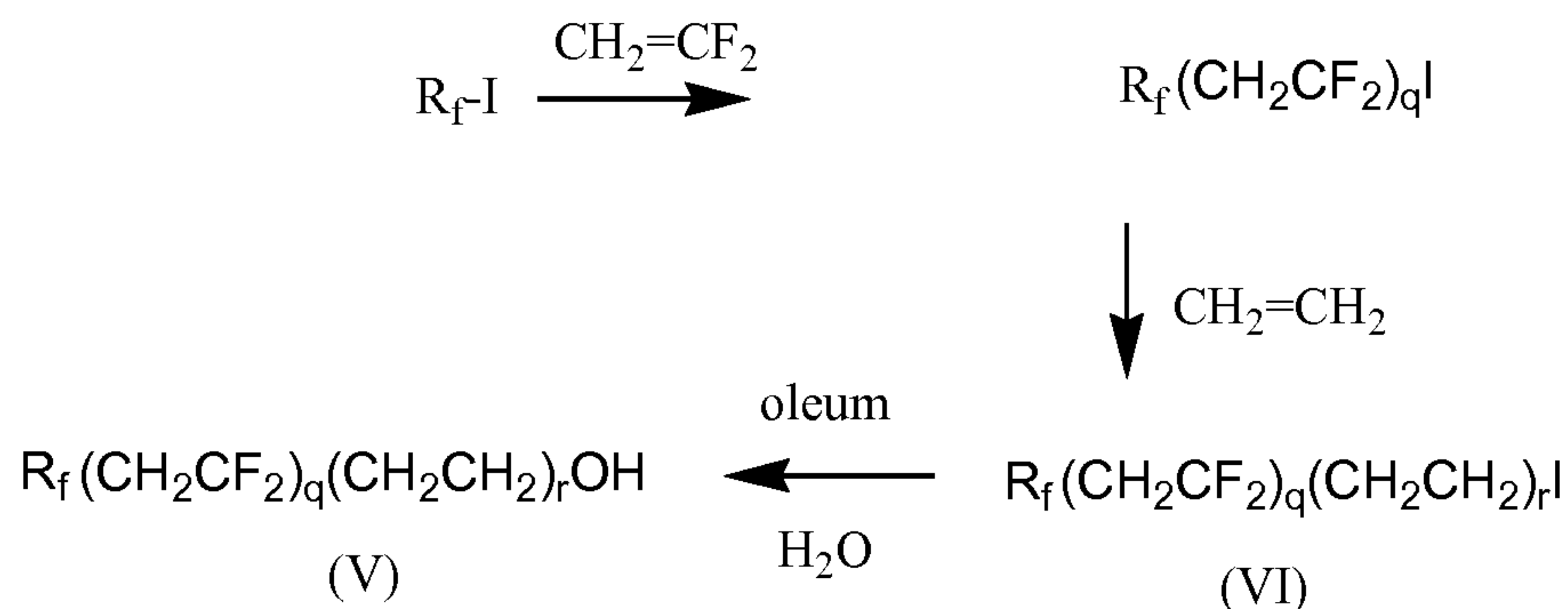
Scheme 1
