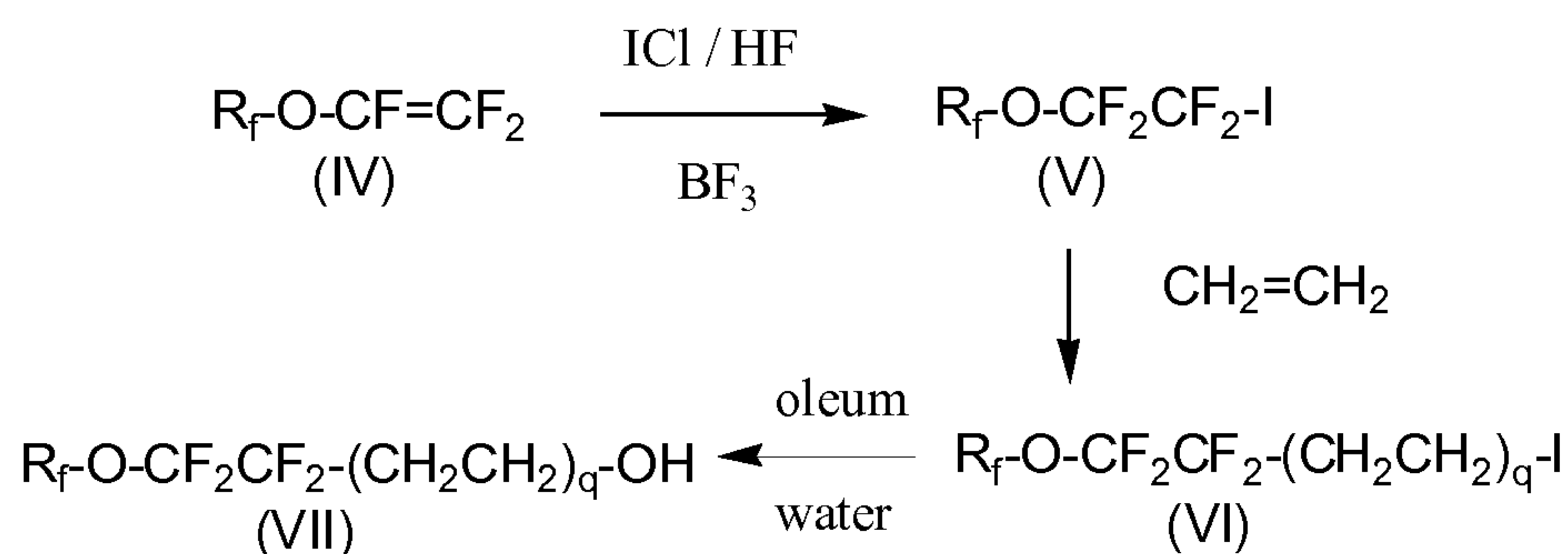
Scheme 2
