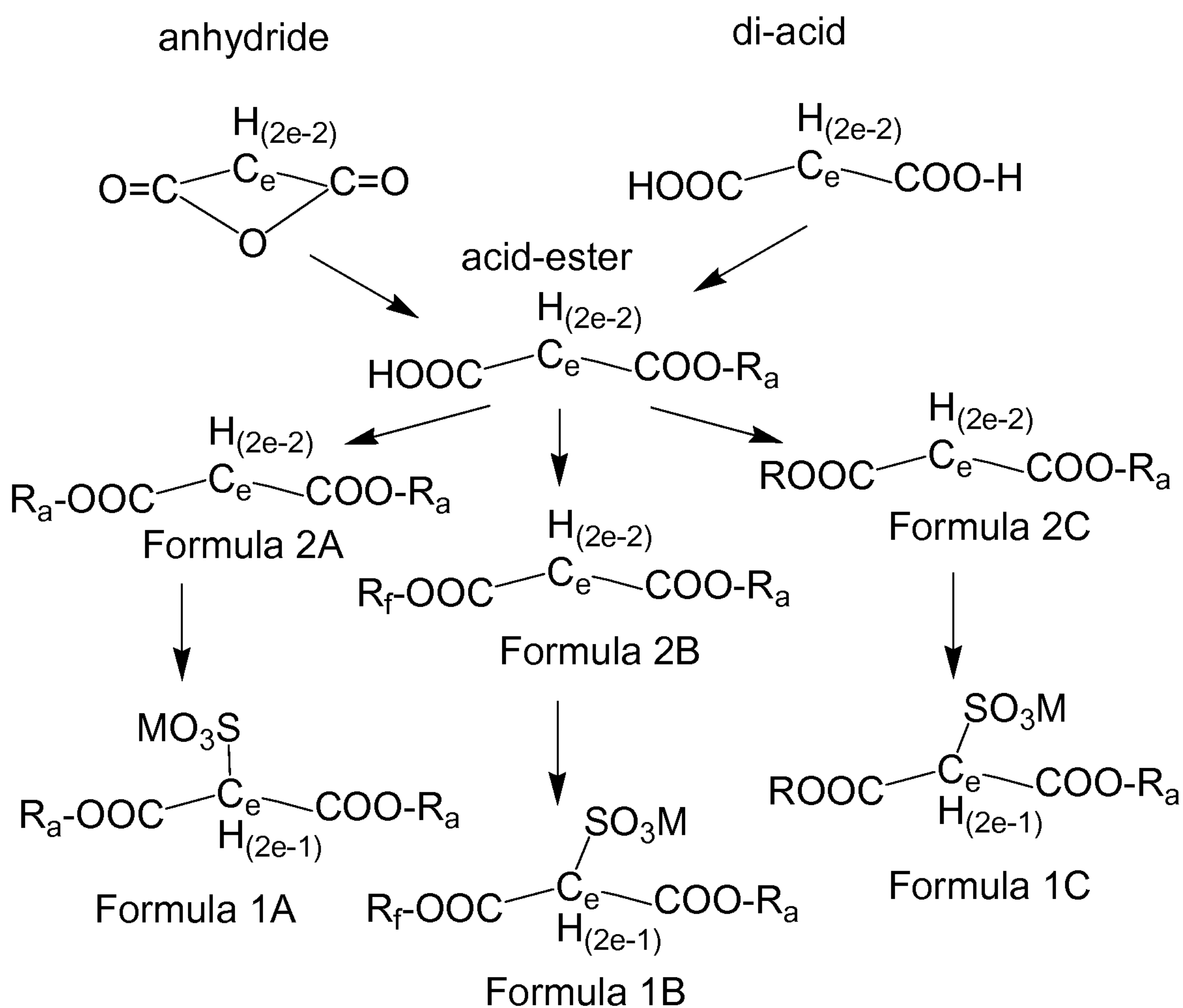
Scheme A
