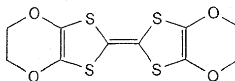
BEDO-TTF
