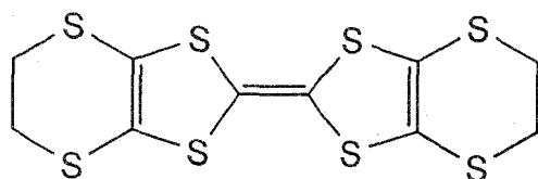
BEDT-TTF
