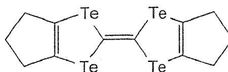
HMTTeF
