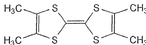
TMTTF
