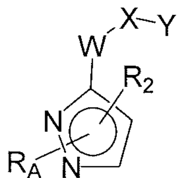
Formula IV
