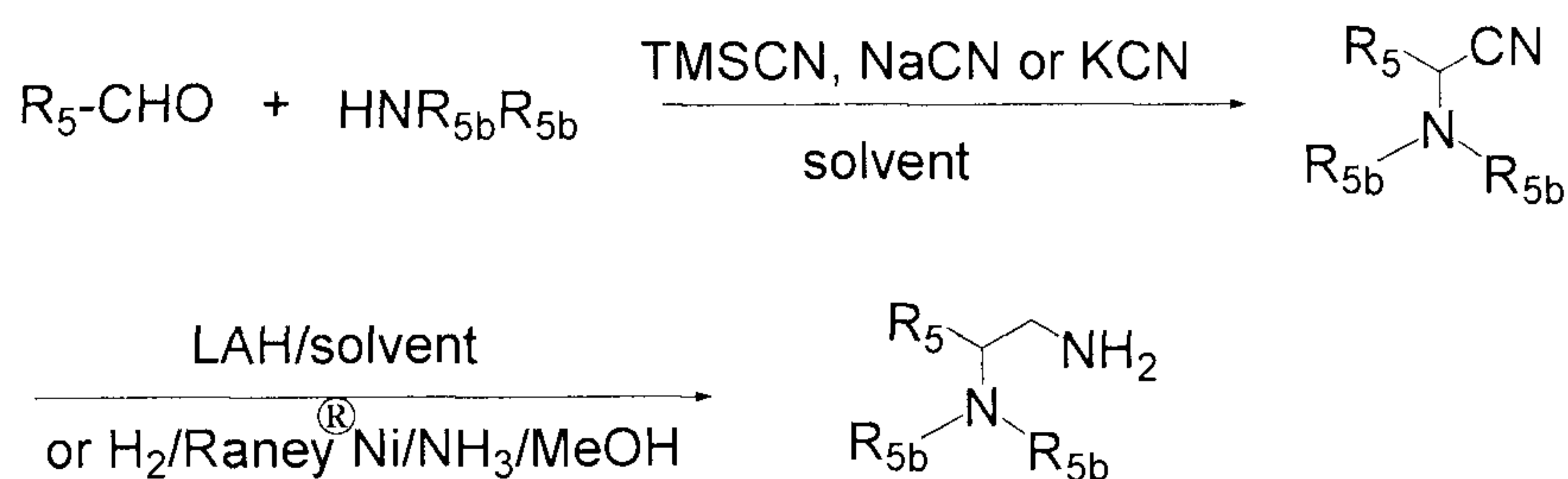
Scheme 16
