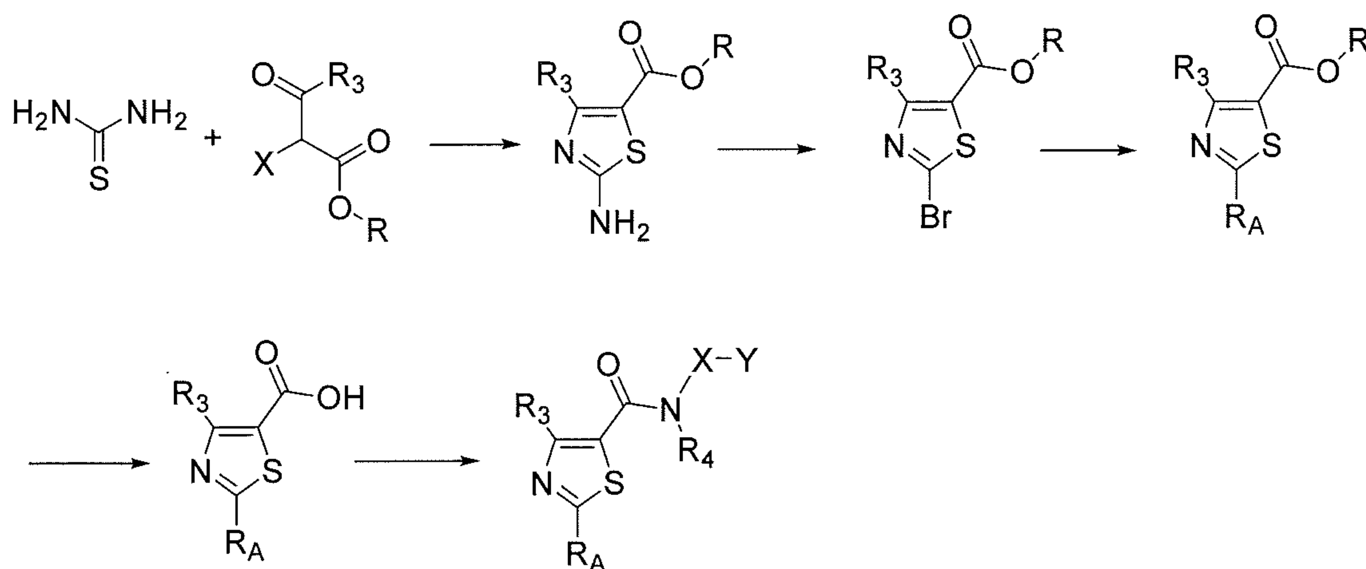
Scheme 7
