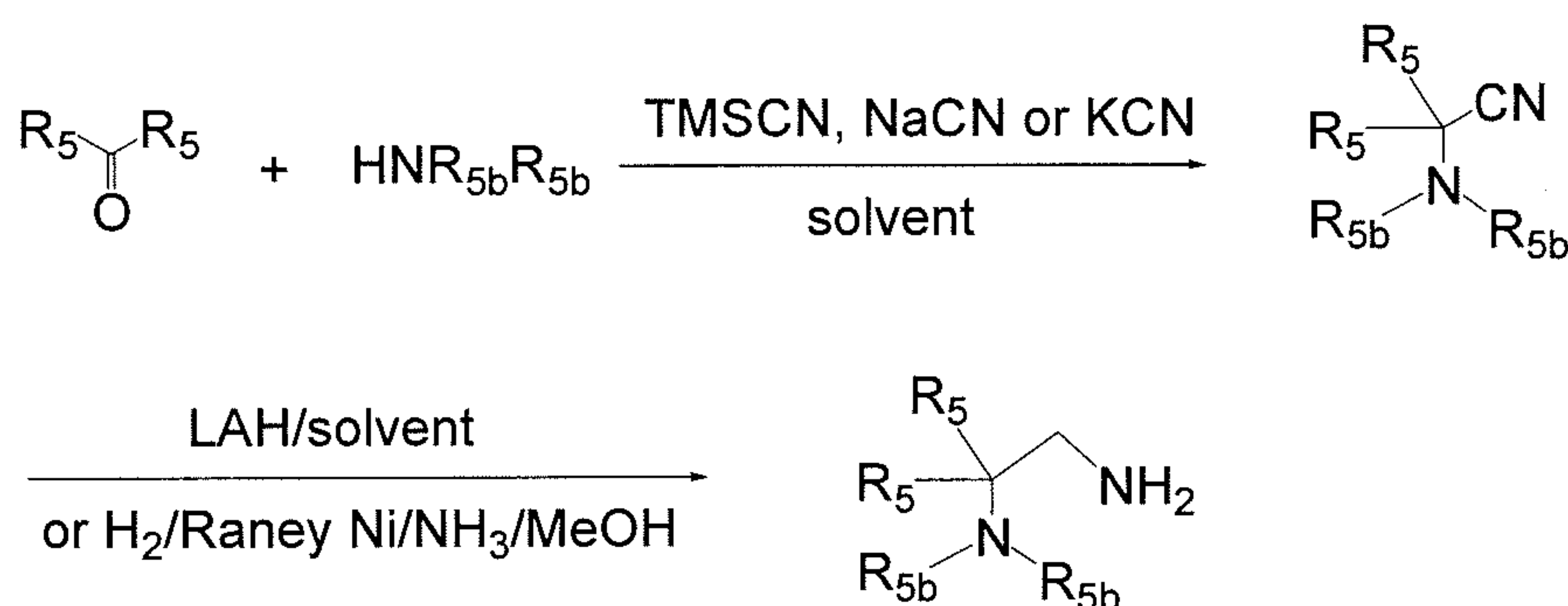
Scheme 18
