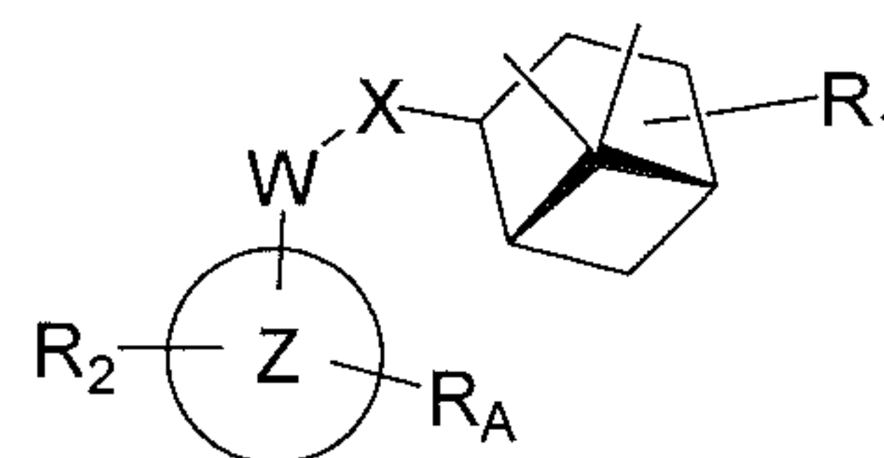
Formula IIc
