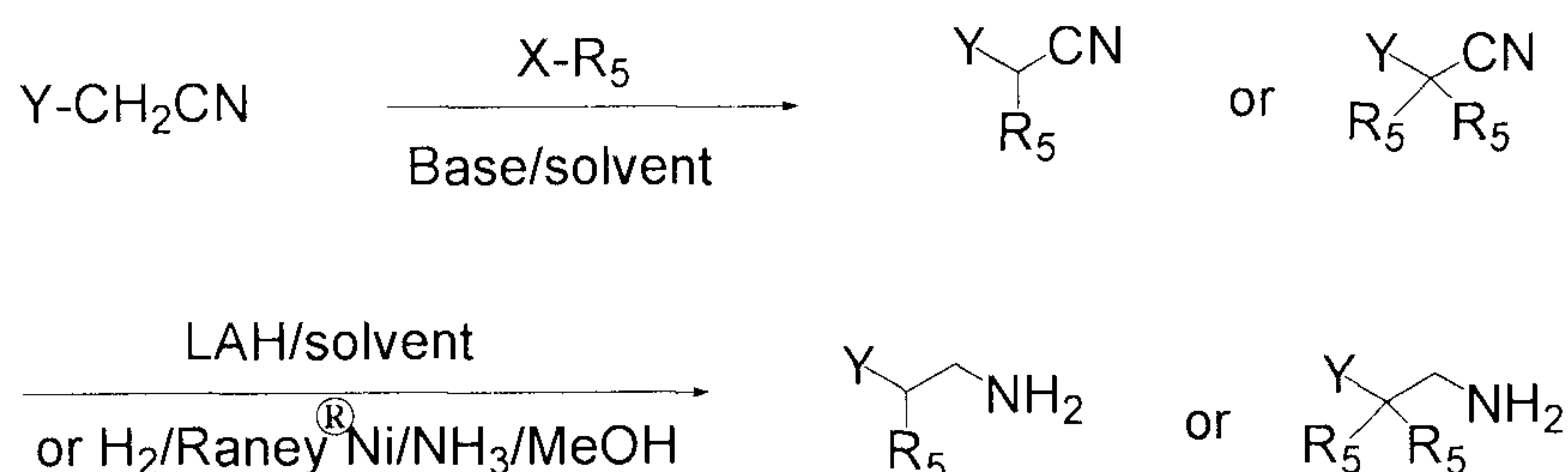
Scheme 17
