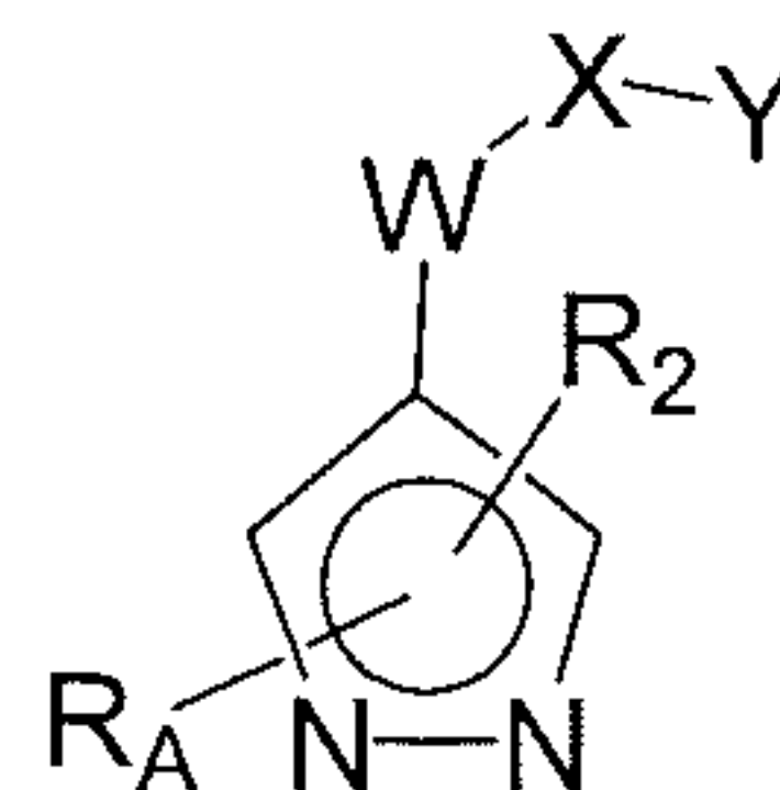
Formula V
