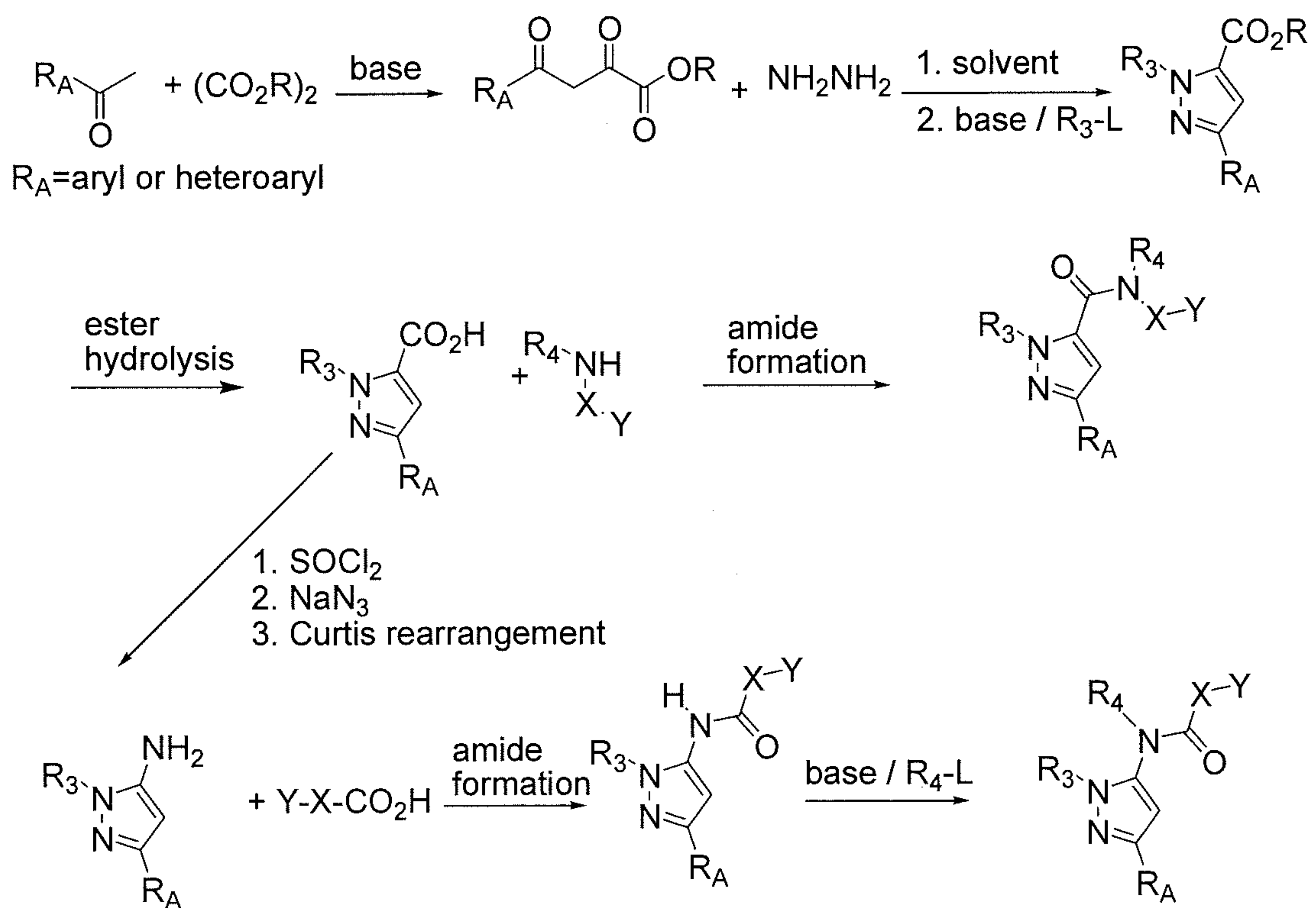
Scheme 11
