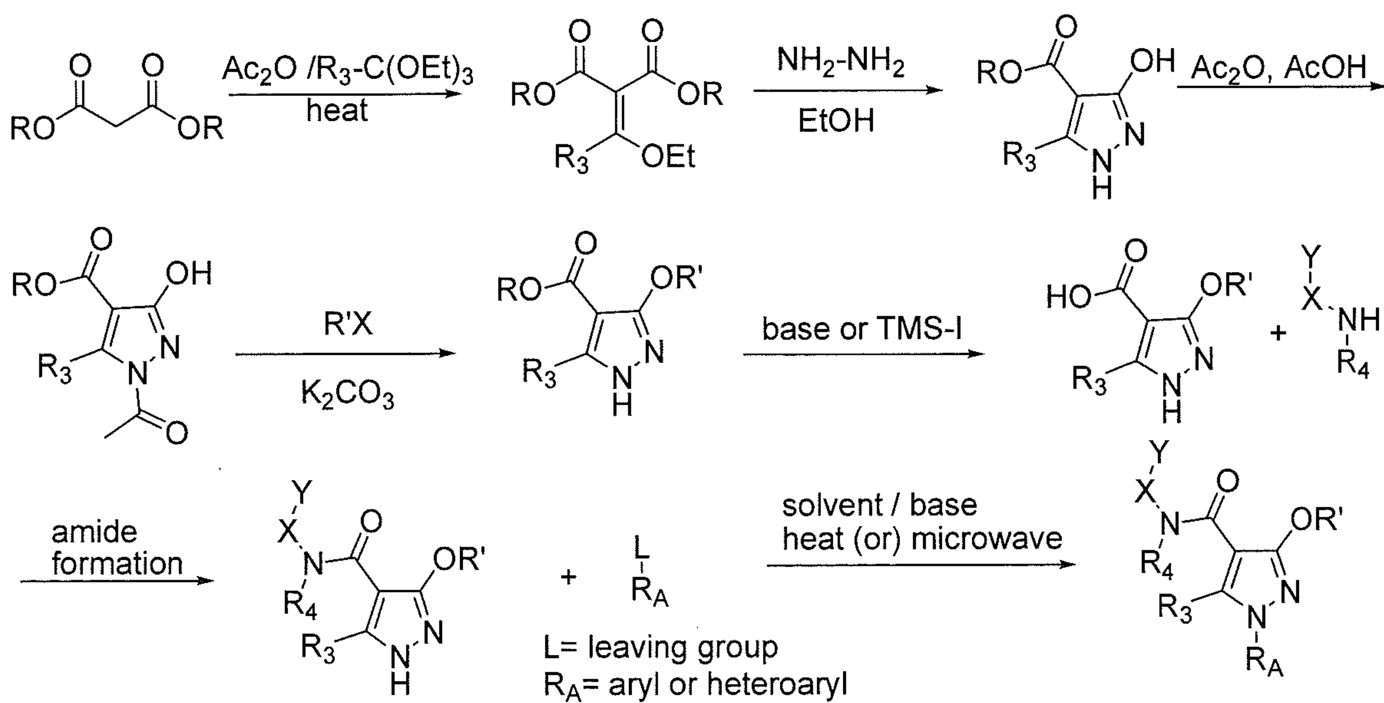
Scheme 2
