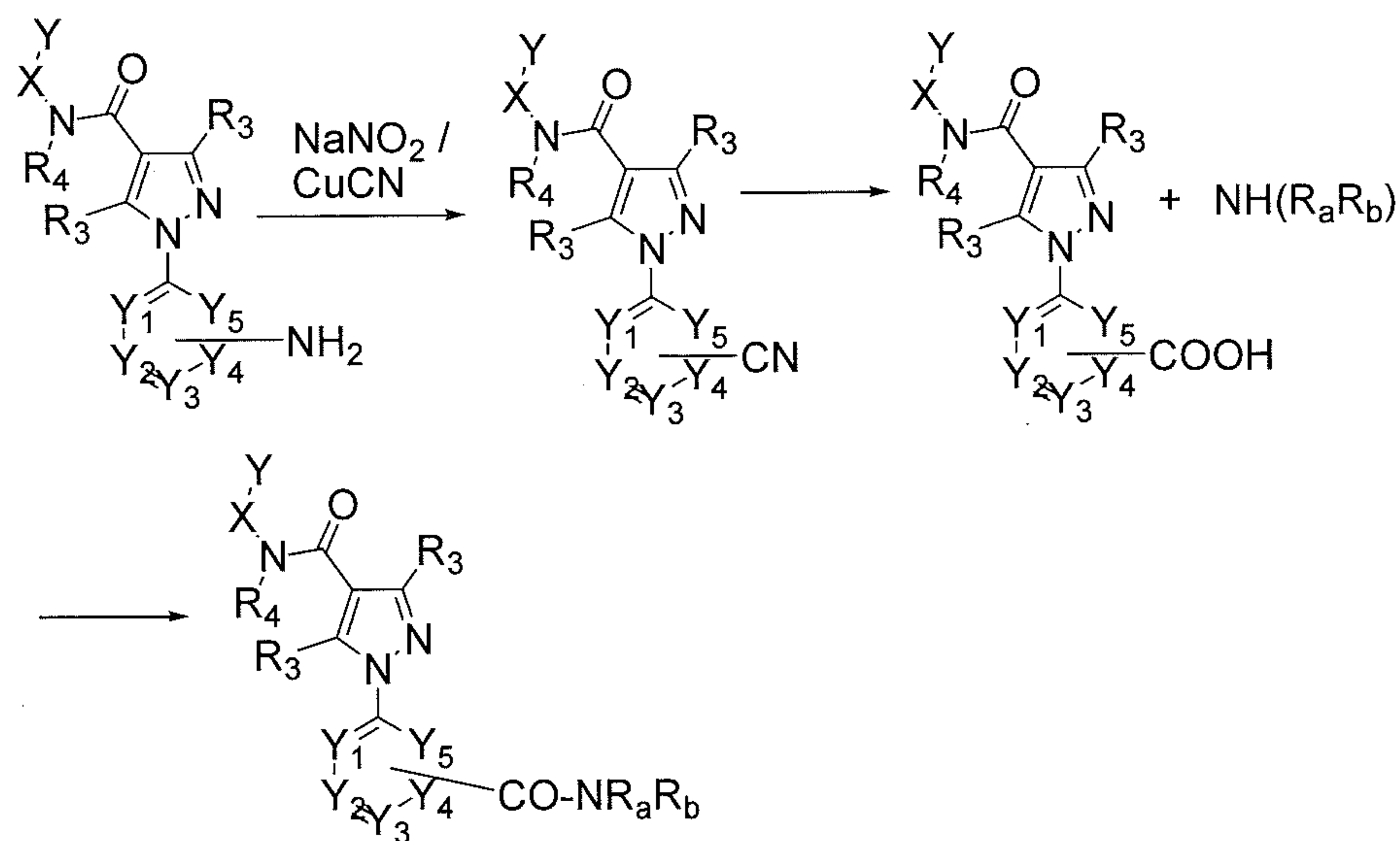
Scheme 4
