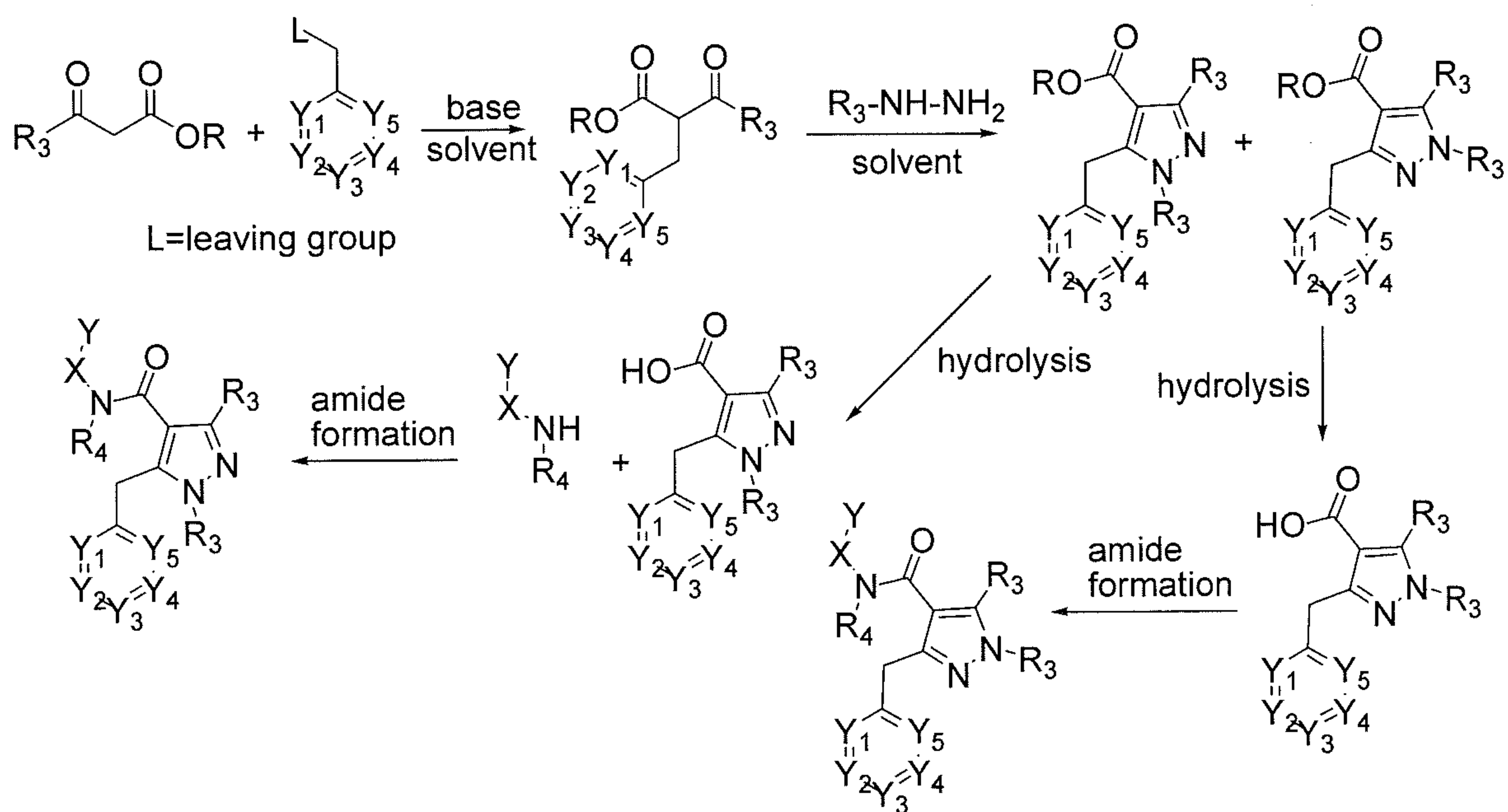
Scheme 5
