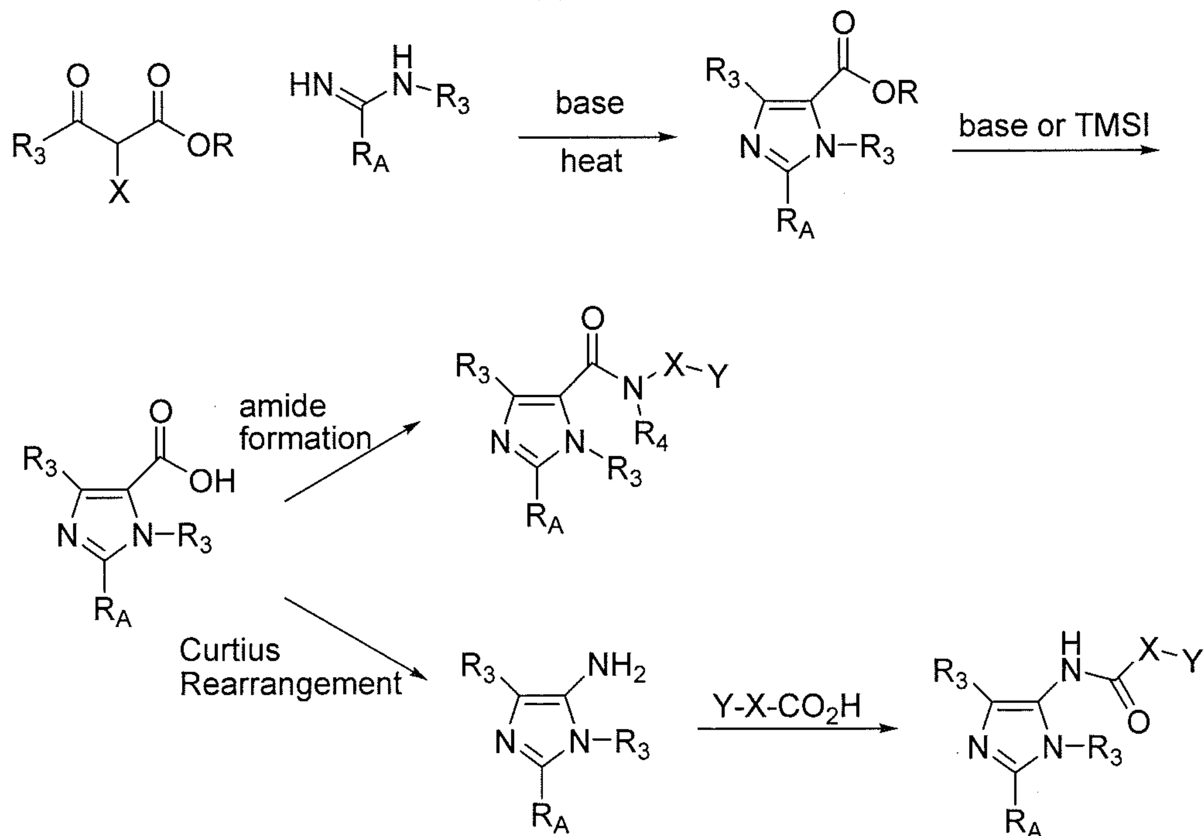
Scheme 9
