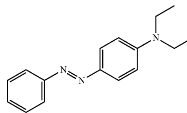
N,N-diethyl-4-[(E)-phenylazo]aniline
