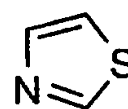
thiazole (thiazolyl)
