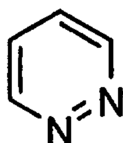
pyridazine (pyridazinyl)
