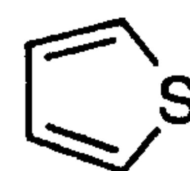
thiophene (thienyl)
