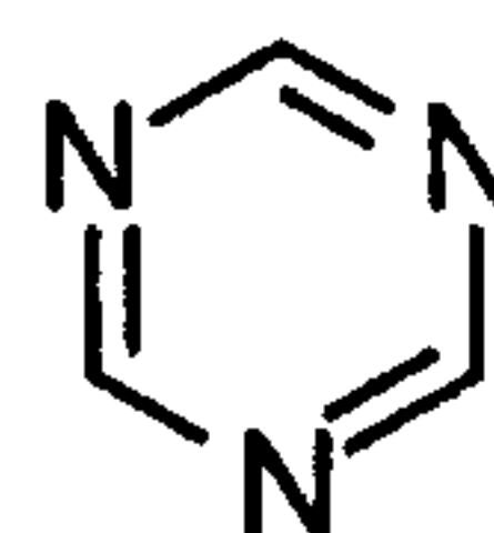
triazine (triazinyl)
