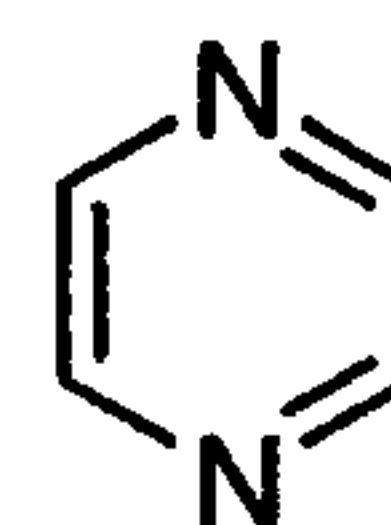
pyrazine (pyrazinyl)
