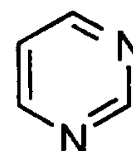
pyrimidine (pyrimidinyl)
