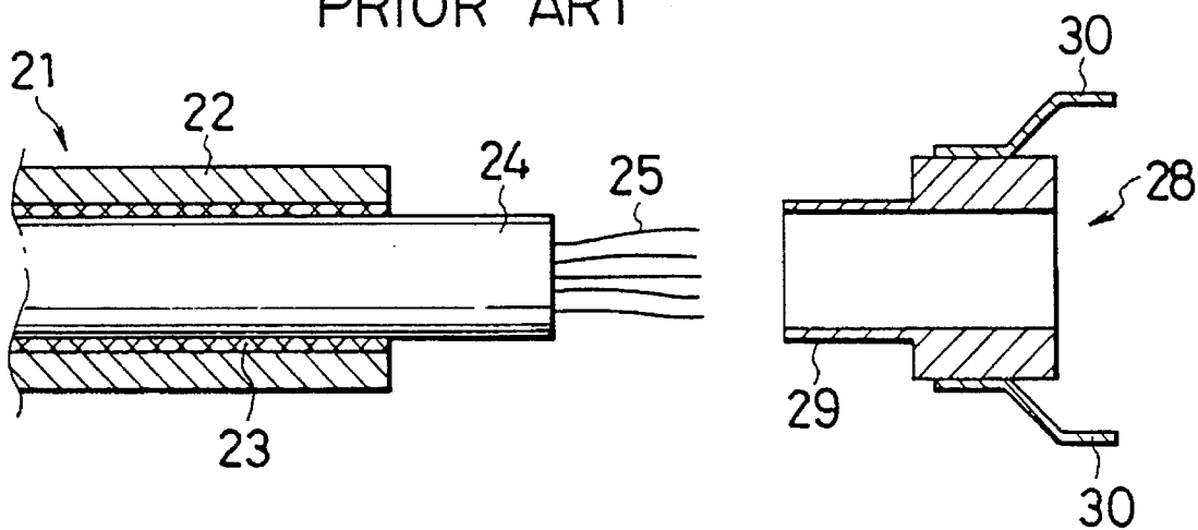
FIG. 5 PRIOR ART
