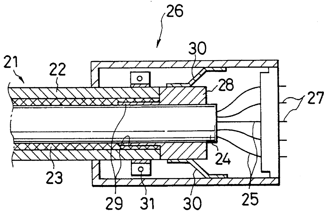
FIG. 4 PRIOR ART
