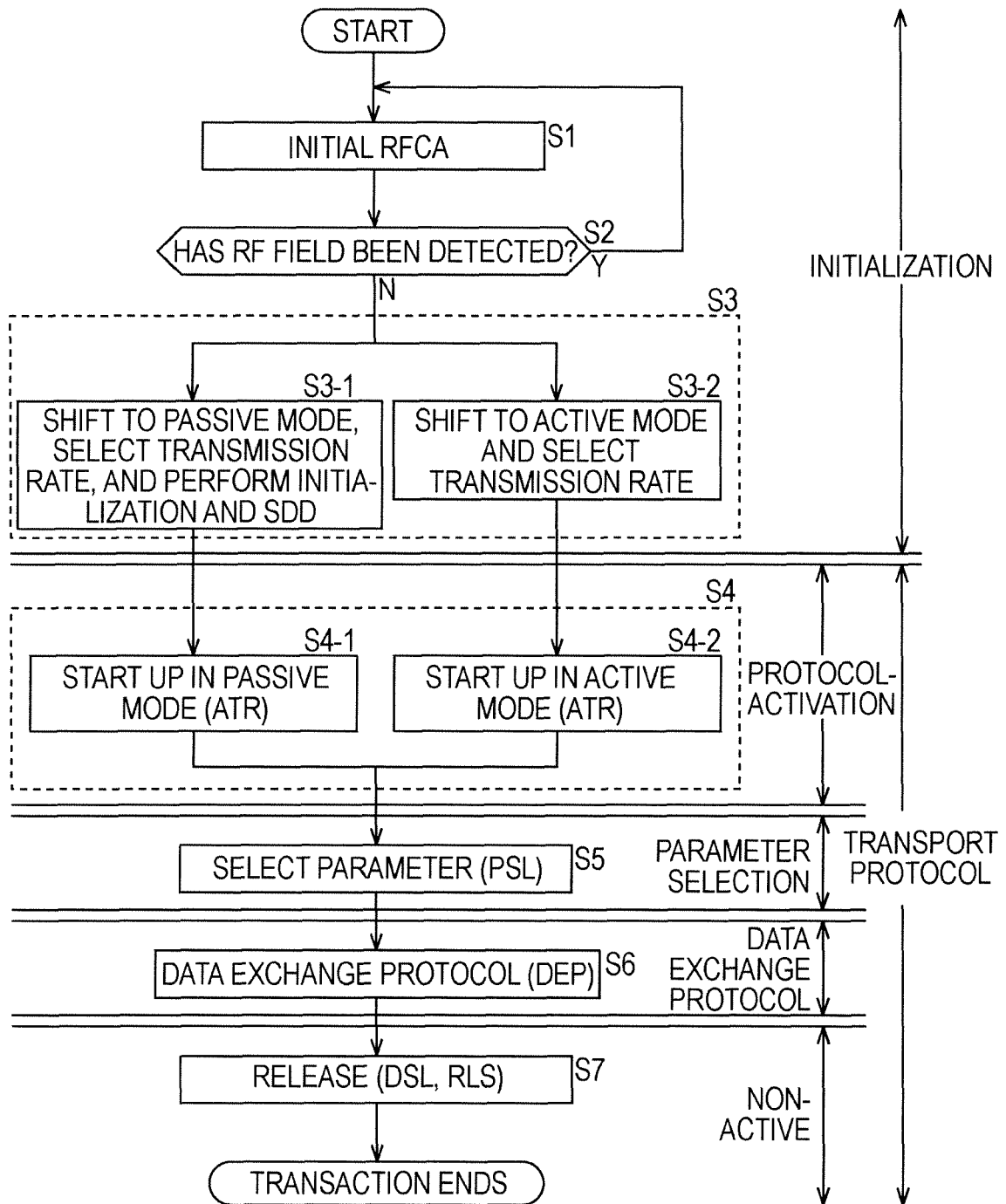
FLOW OF INITIALIZATION AND SDD
