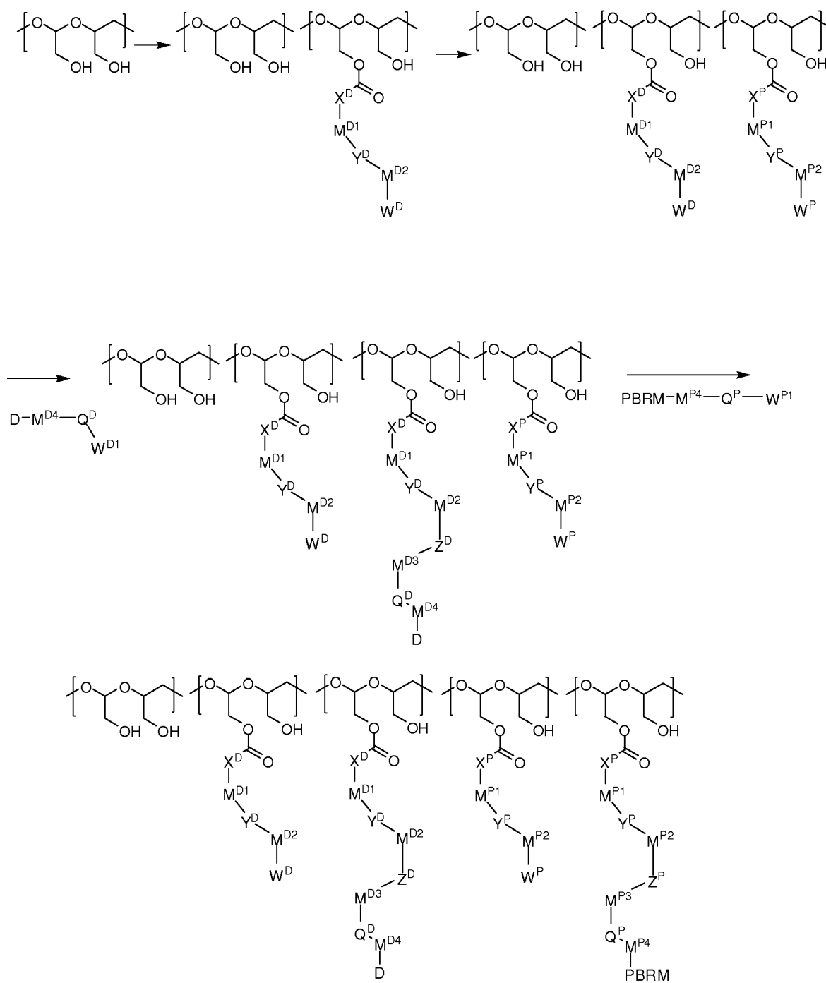
Scheme 5A
