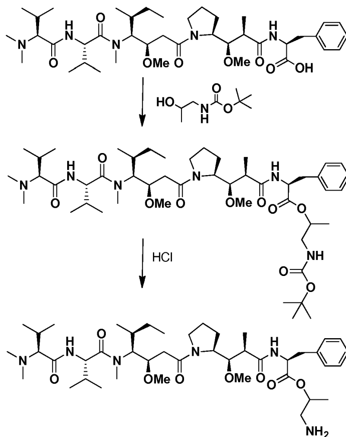
Scheme 4
