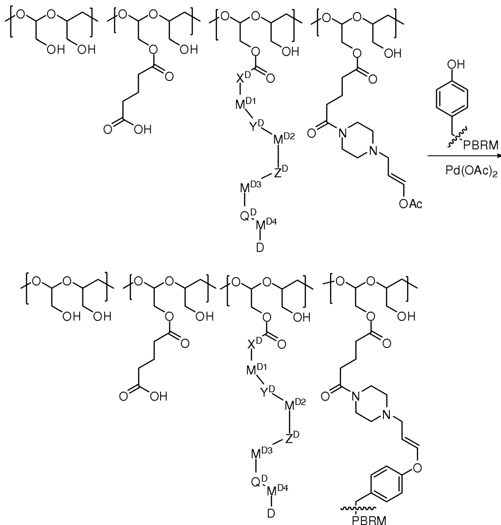
Scheme 9
