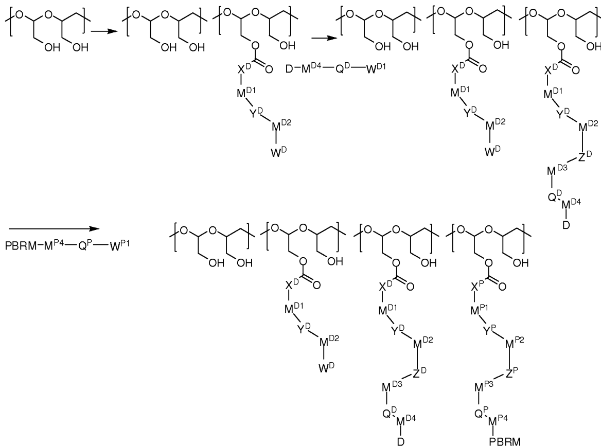
Scheme 6
