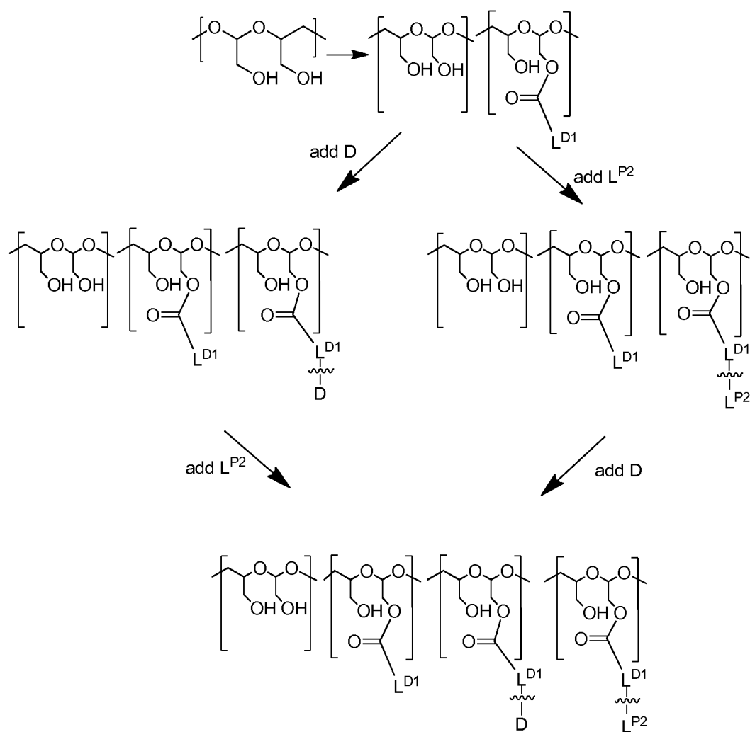
Scheme 10
