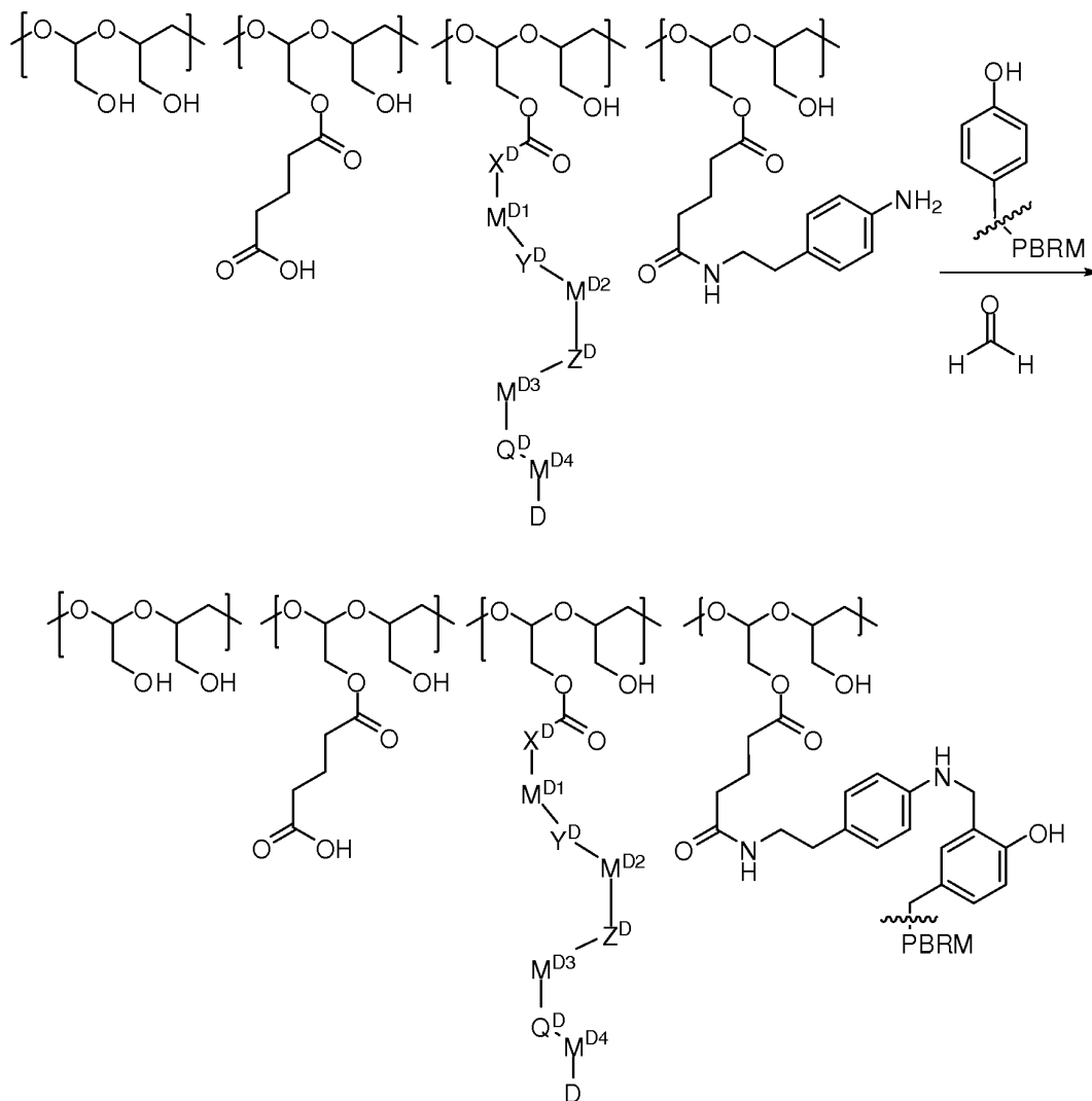
Scheme 8
