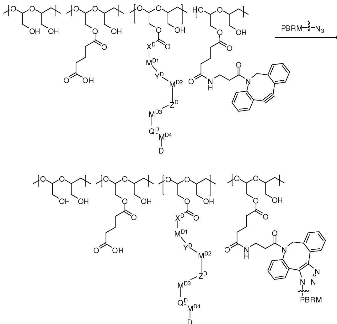
Scheme 7
