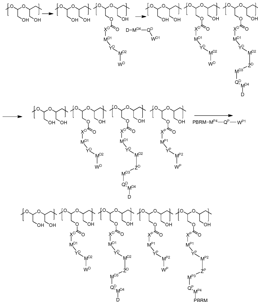
Scheme 5
