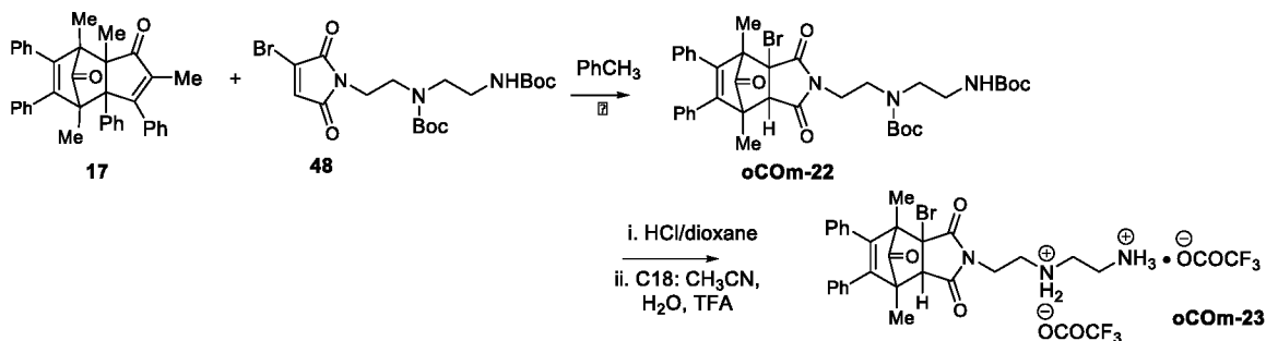
Scheme 22a: Synthesis of oCom-23 as its trifluoroacetic acid salt.
