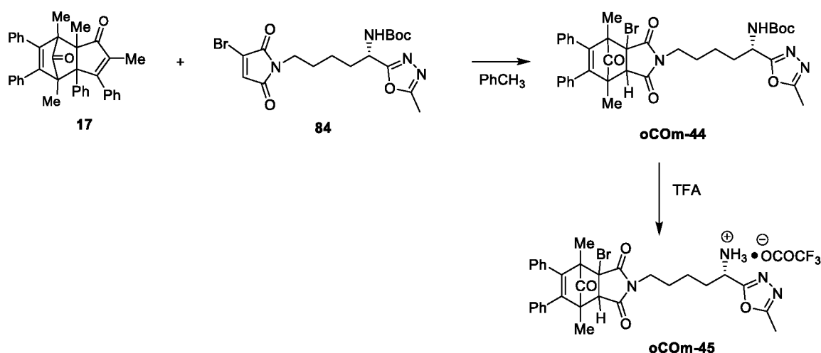
Scheme 34: Synthesis of oCom-44 and -45
