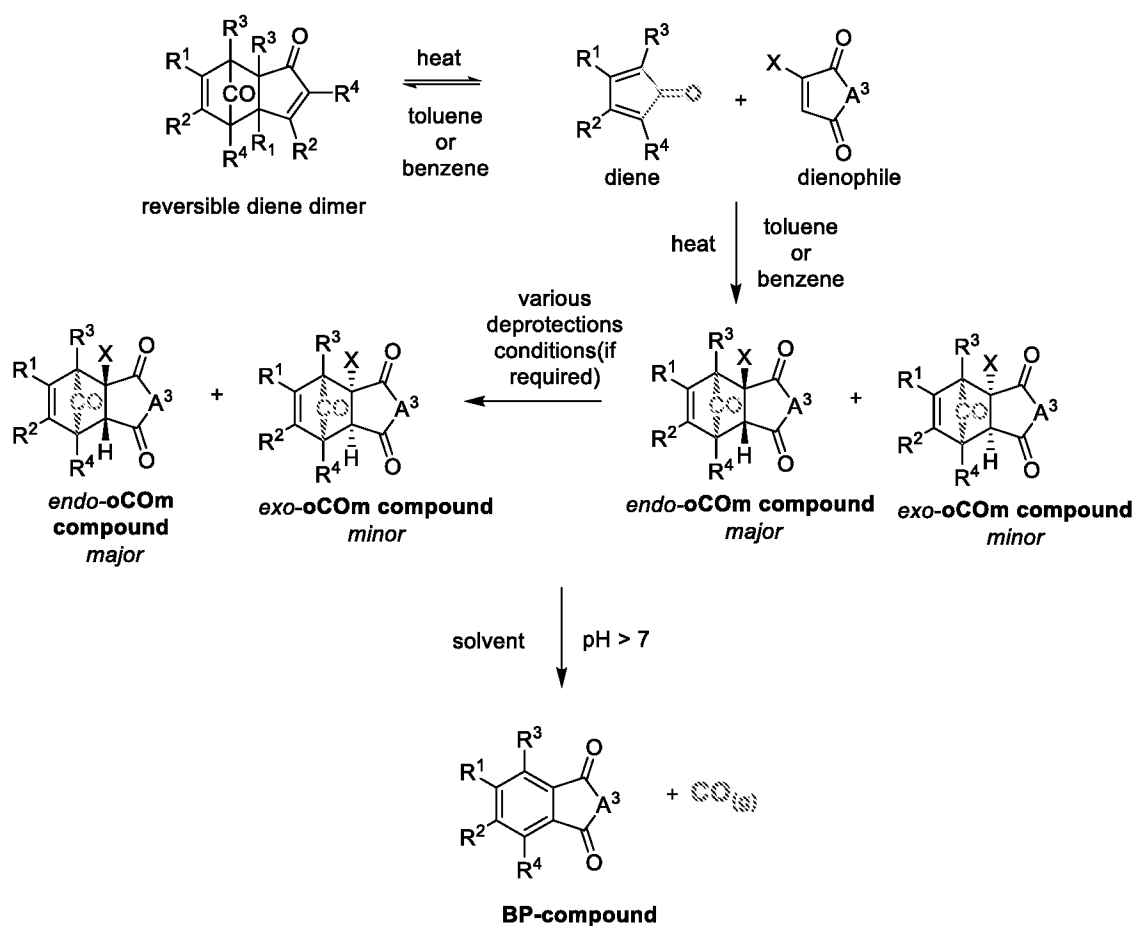
10 Scheme 2: Procedure for preparing Norbornenone Compound with the Formula 1a(i)
