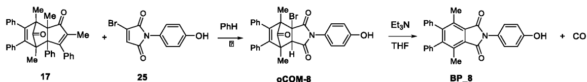
Scheme 11: Synthesis of oCOM-8 and base promoted release of carbon monoxide forming BP-8
