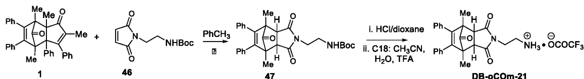
Scheme 21b: Synthesis of control compound DB-oCOM-21 as the hydrochloride and trifluoroacetic acid salts.
