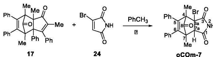
Scheme 10: Synthesis of oCOM-7
