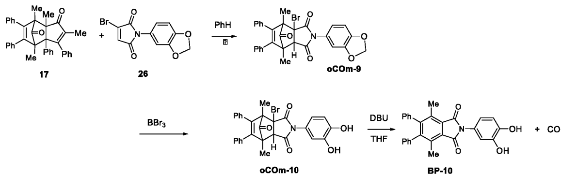
Scheme 12: Synthesis of oCOM-10 and base promoted release of carbon monoxide forming BP-10
