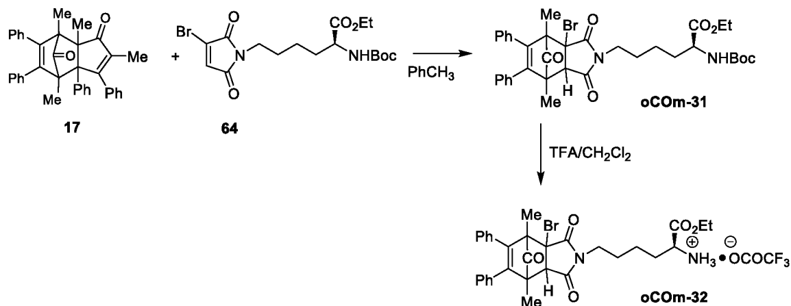
Scheme 27: Synthesis of oCOM-31 and -32
