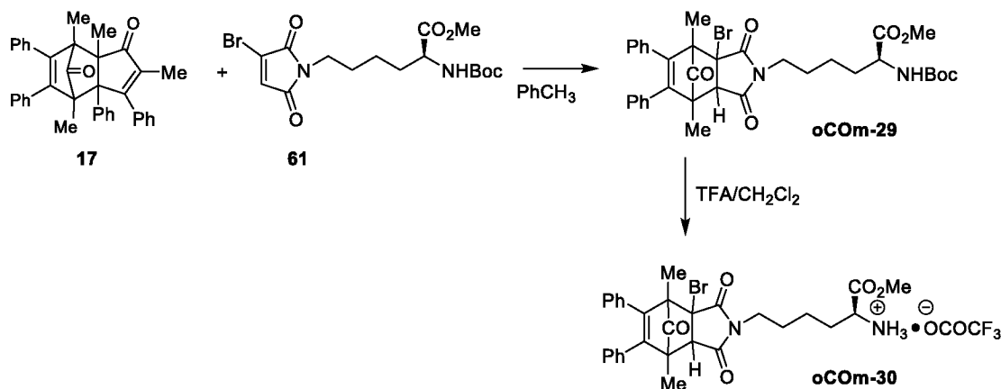
Scheme 26: Synthesis of oCom-29 and -30
