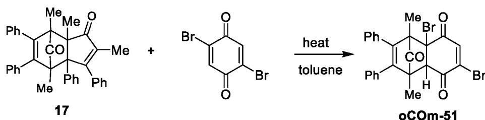
Scheme 3: Preparation of oCom-51
