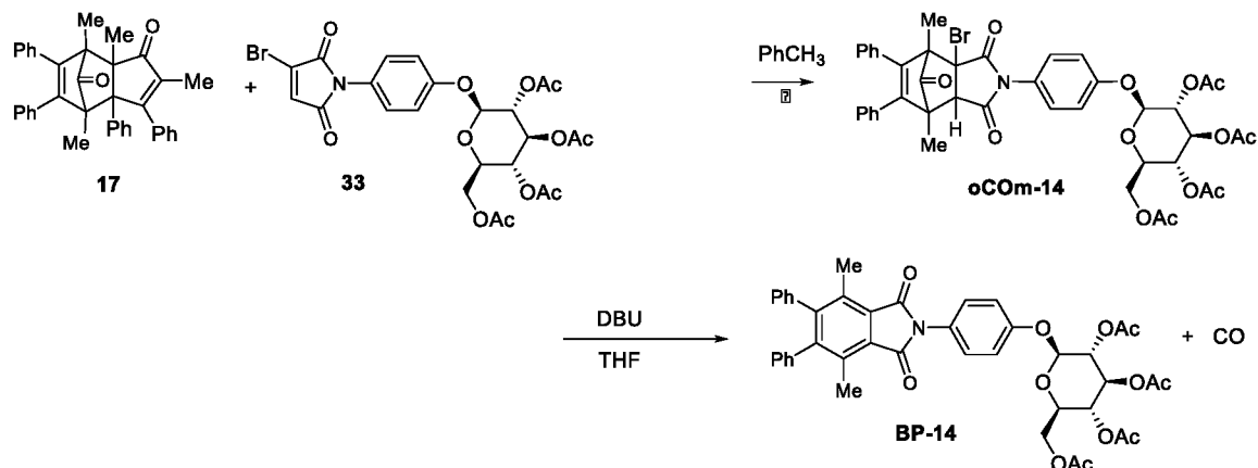
Scheme 16: Synthesis of oCOM-14 and base promoted release of carbon monoxide forming BP-14
