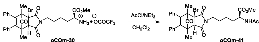
Scheme 32: Synthesis of oCom-41
