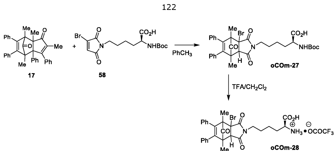
Scheme 25: Synthesis of oCom-27 and -28
