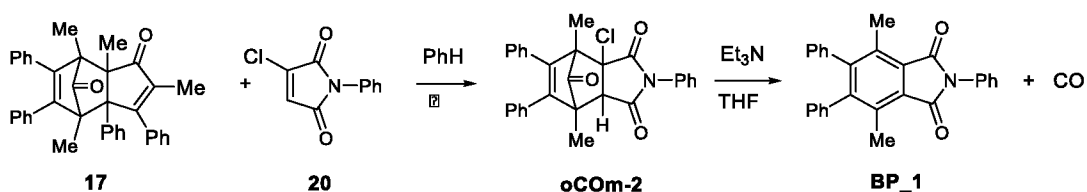
Scheme 5: Synthesis of oCOM-2 and base promoted release of carbon monoxide forming BP-1
