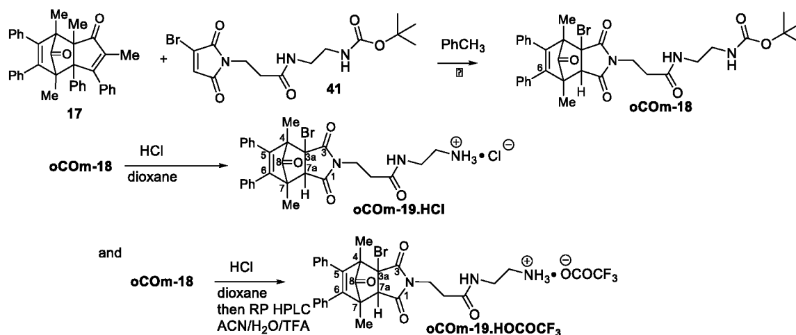
Scheme 20: Synthesis of oCom-19 as the hydrochloride and trifluoroacetic acid salts.
