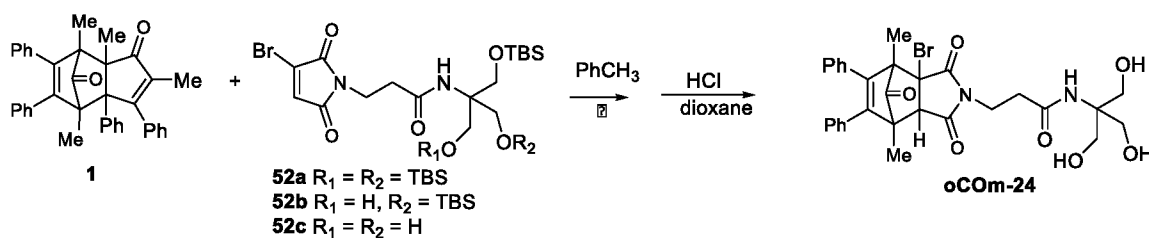
Scheme 23a: Synthesis of oCom-24 .
