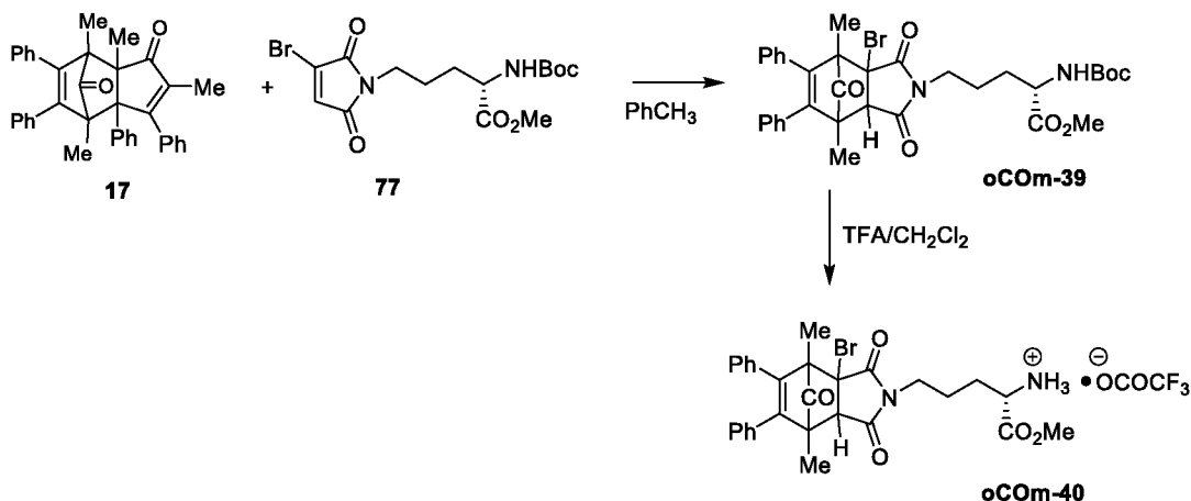
Scheme 31: Synthesis of oCOM-39 and -40
