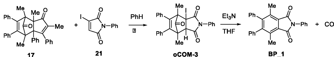
Scheme 6: Synthesis of oCOM-3 and base promoted release of carbon monoxide forming BP-1
