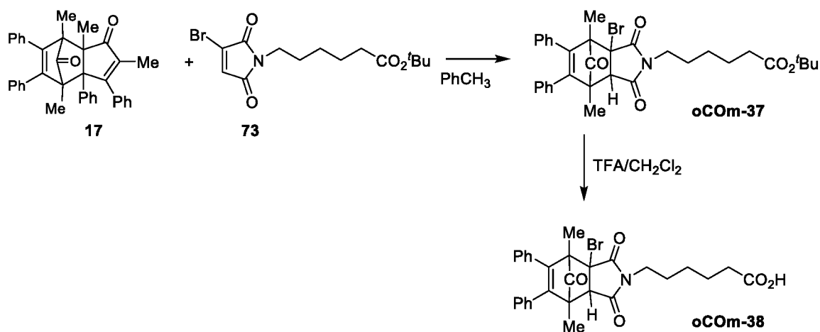
Scheme 30: Synthesis of oCOM-37 and -38
