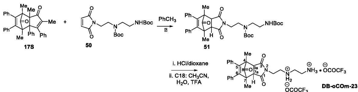
Scheme 22b: Synthesis of control compound DB-oCom-23 as its trifluoroacetic acid salt.
