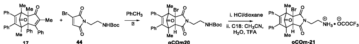
Scheme 21a: Synthesis of oCom-21 as its trifluoroacetic acid salt.
