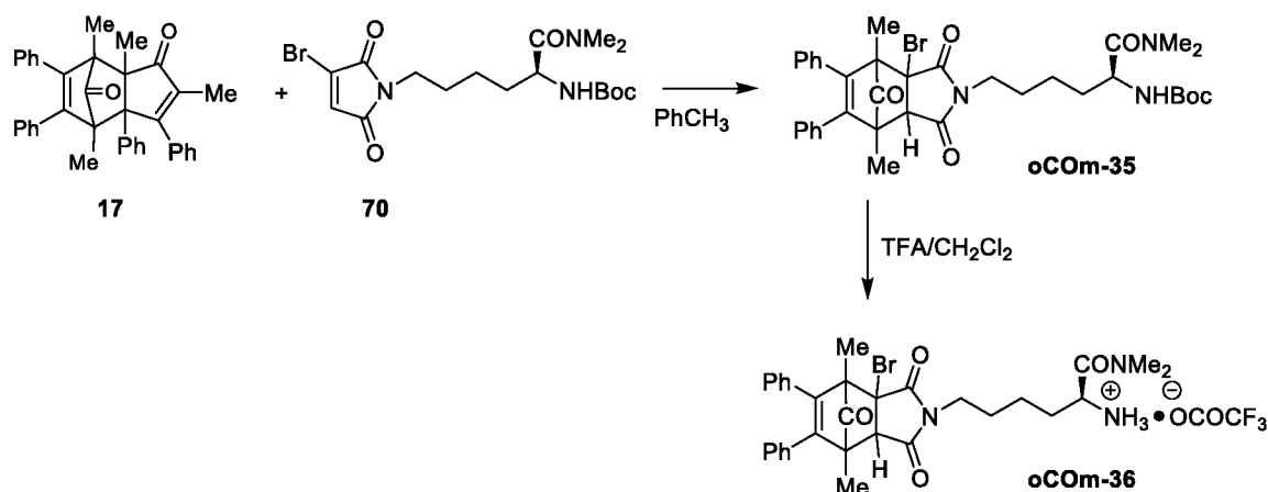
Scheme 29: Synthesis of oCom-35 and -36
