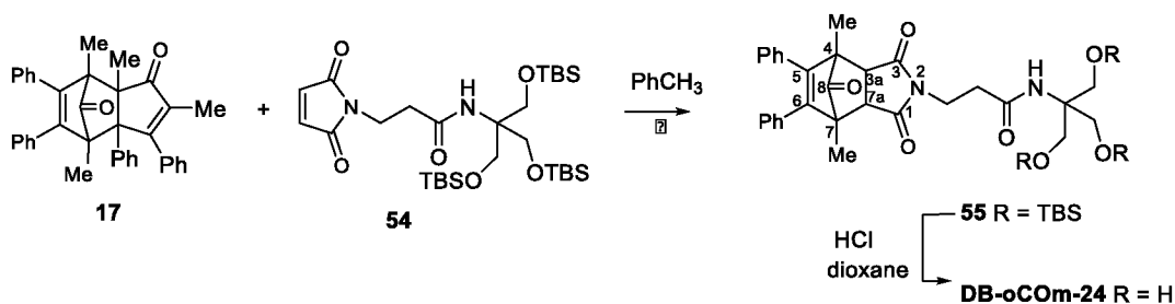
Scheme 23b: Synthesis of control compound DB-oCOM-24 .
