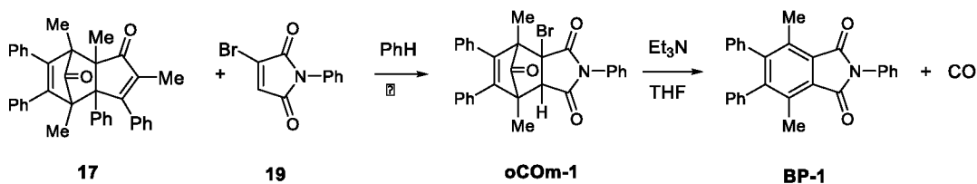
Scheme 4: Synthesis of oCOM-1 and base promoted release of carbon monoxide forming BP-1
