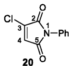
Scheme 5: Synthesis of oCOM-2 and base promoted release of carbon monoxide forming BP-1
