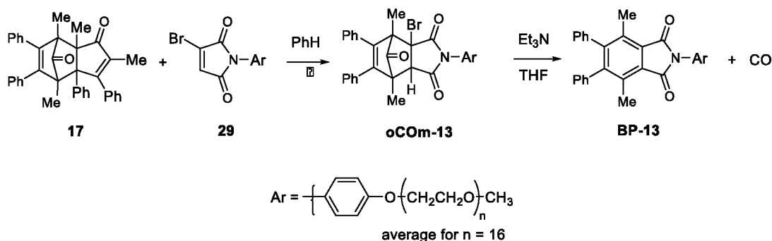
Scheme 15: Synthesis of oCOM-13 and base promoted release of carbon monoxide forming BP-13
