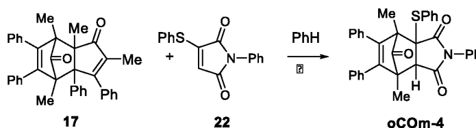
Scheme 7: Synthesis of oCom-4
