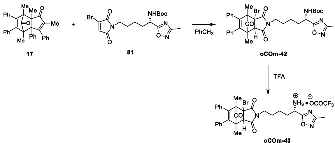
Scheme 33: Synthesis of oCom-42 and -43
