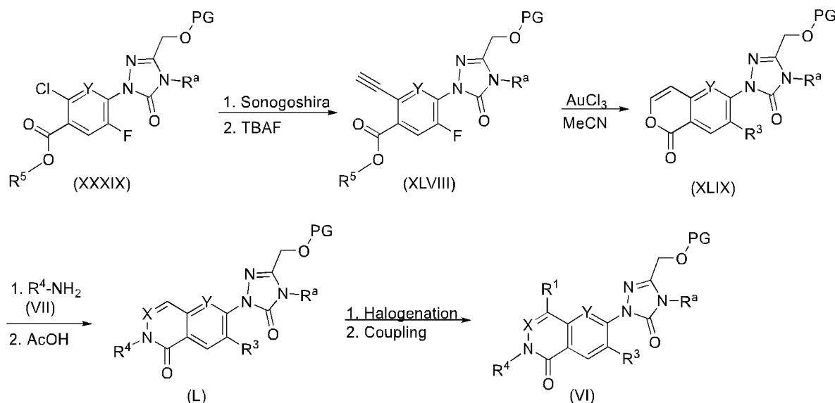
SCHEME 23
