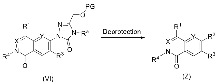
SCHEME 24
