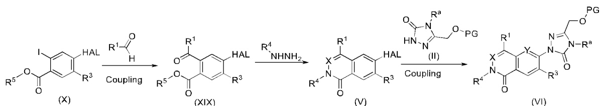
SCHEME 9
