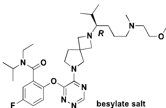
Compound A4-a
