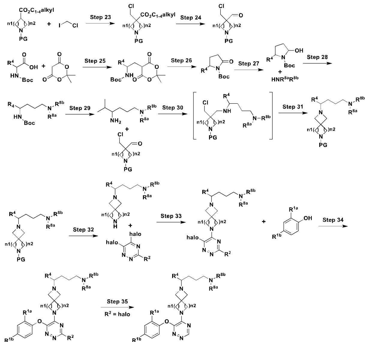
Scheme 9
