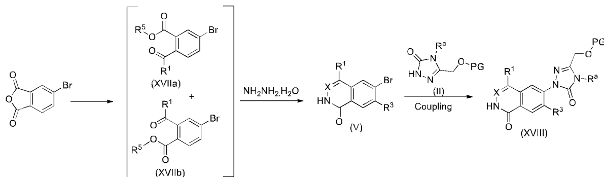
SCHEME 8
