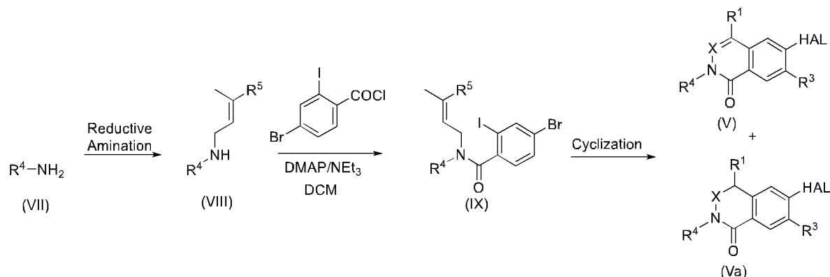
SCHEME 4
