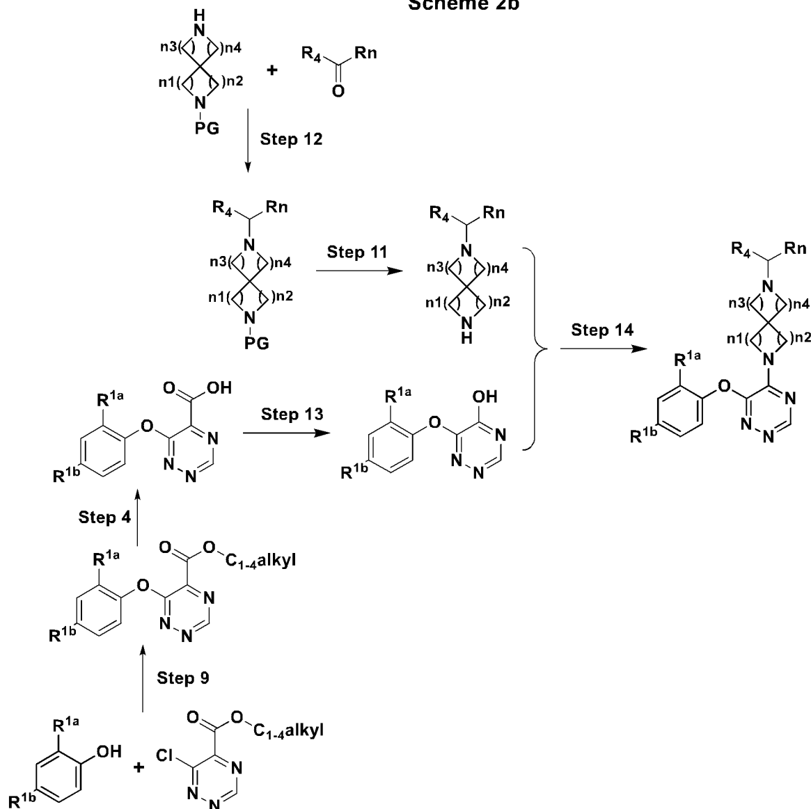
Scheme 2b
