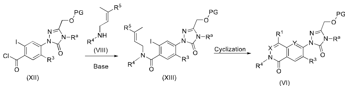
SCHEME 6
