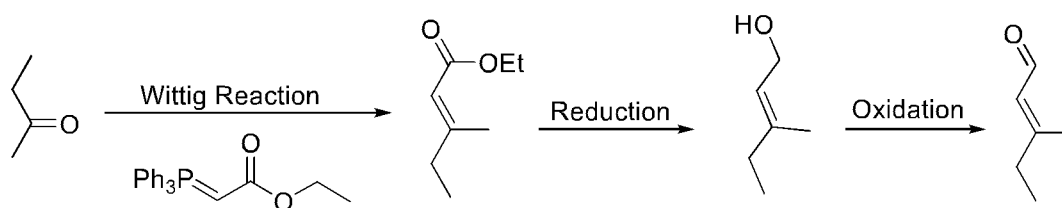
SCHEME 15
