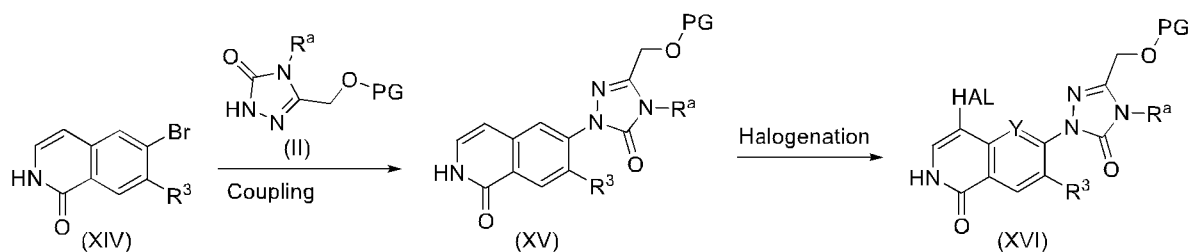
SCHEME 7
