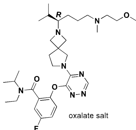
Compound A3.
