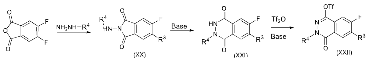
SCHEME 11
