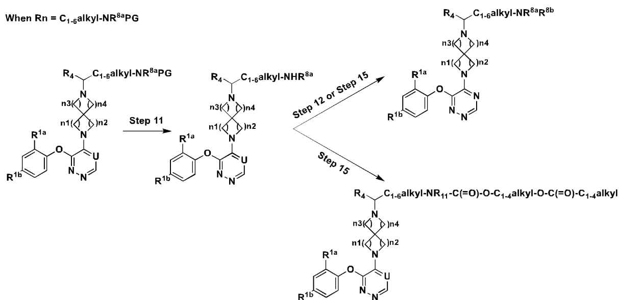
Scheme 3
