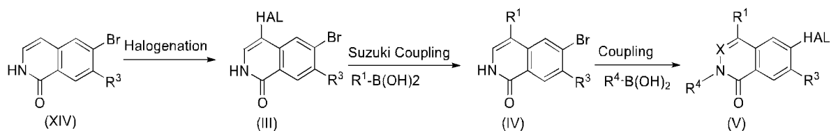
SCHEME 2
