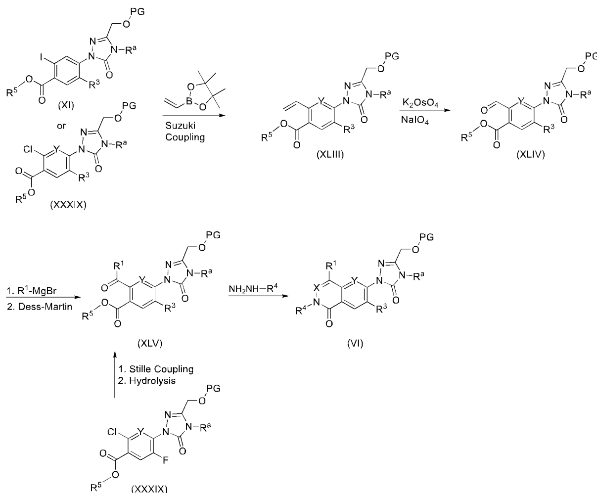
SCHEME 21
