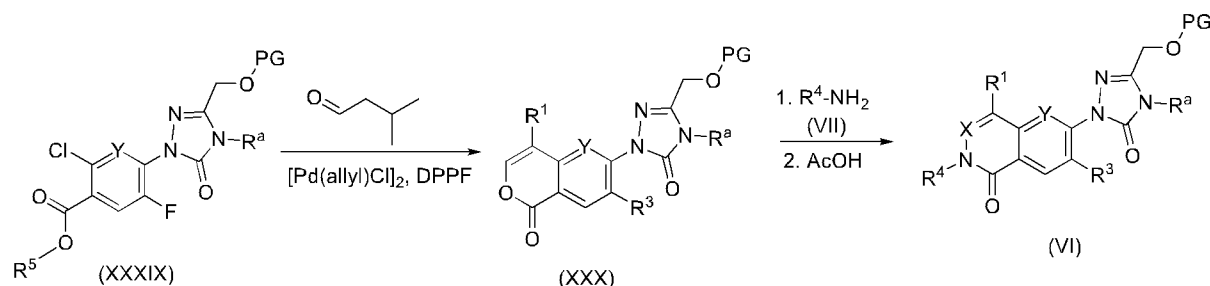
SCHEME 20
