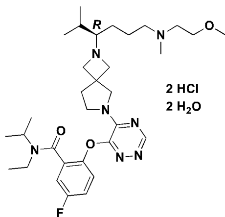
Compound A2.
