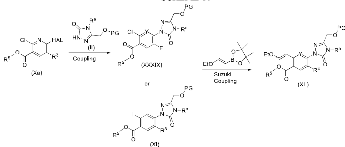
SCHEME 18
