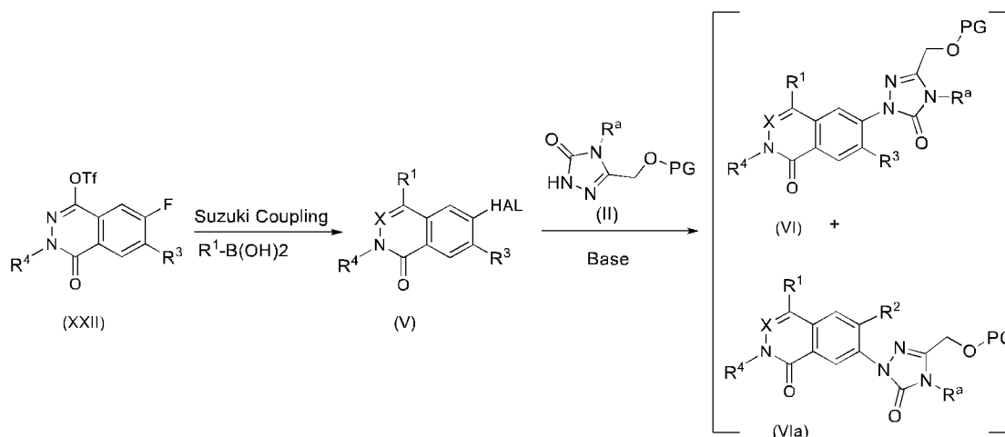
SCHEME 12
