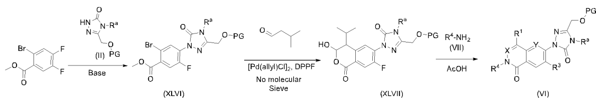
SCHEME 22
