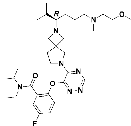
Compound A
