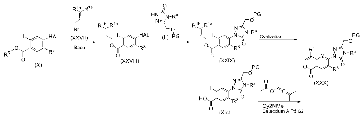
SCHEME 14
