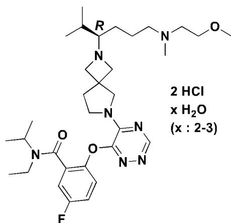
Compound A1.
