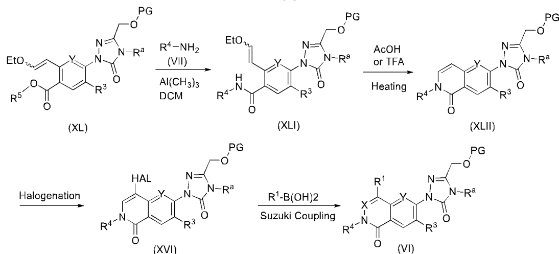
SCHEME 19
