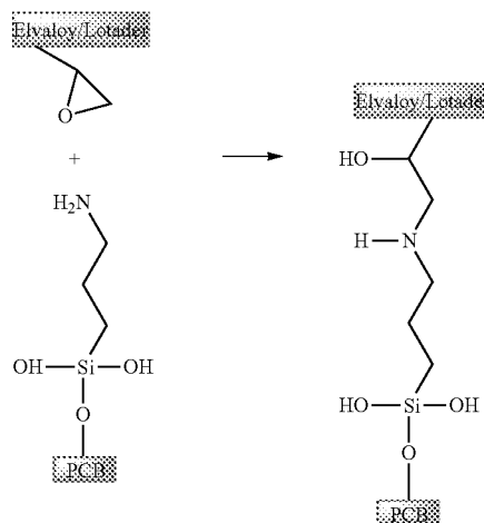
Example 6: Bonding Thermoplastic Material to the PCB
