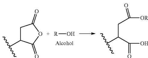
Scheme 9-2.
