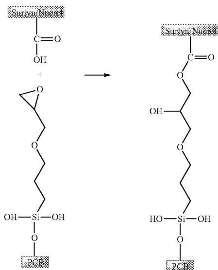
Example 4: Bonding Thermoplastic Material to the PCB
