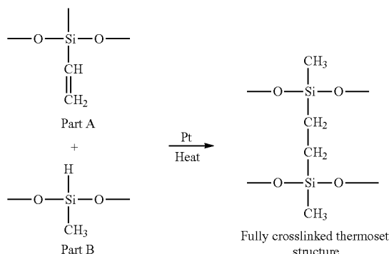
Scheme 11.
