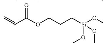
(3-acryloxypropyl)trimethoxysilane
