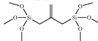
1,1-bis(trimethoxysilylmethyl)ethylene
