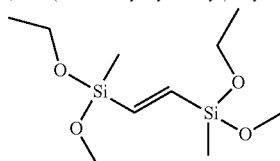
1,2-bis(methyldiethoxysilyl)ethylene
