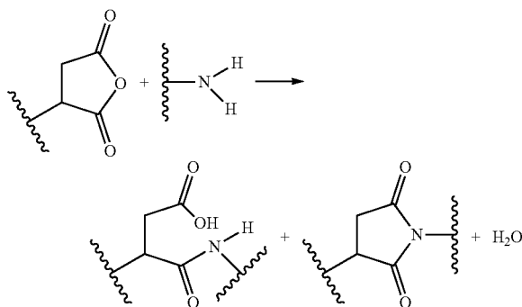
Scheme 9-1.
