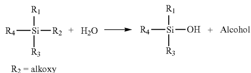
Scheme 10-1.
