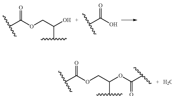
Scheme 7-2.
