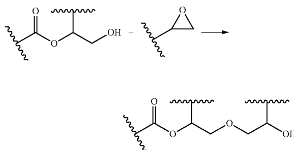
Scheme 7-1.
