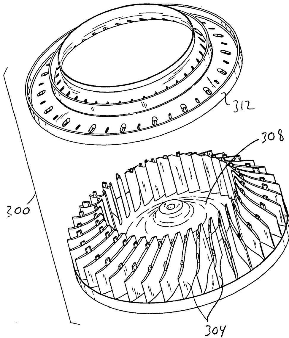
FIG. 1c PRIOR ART
