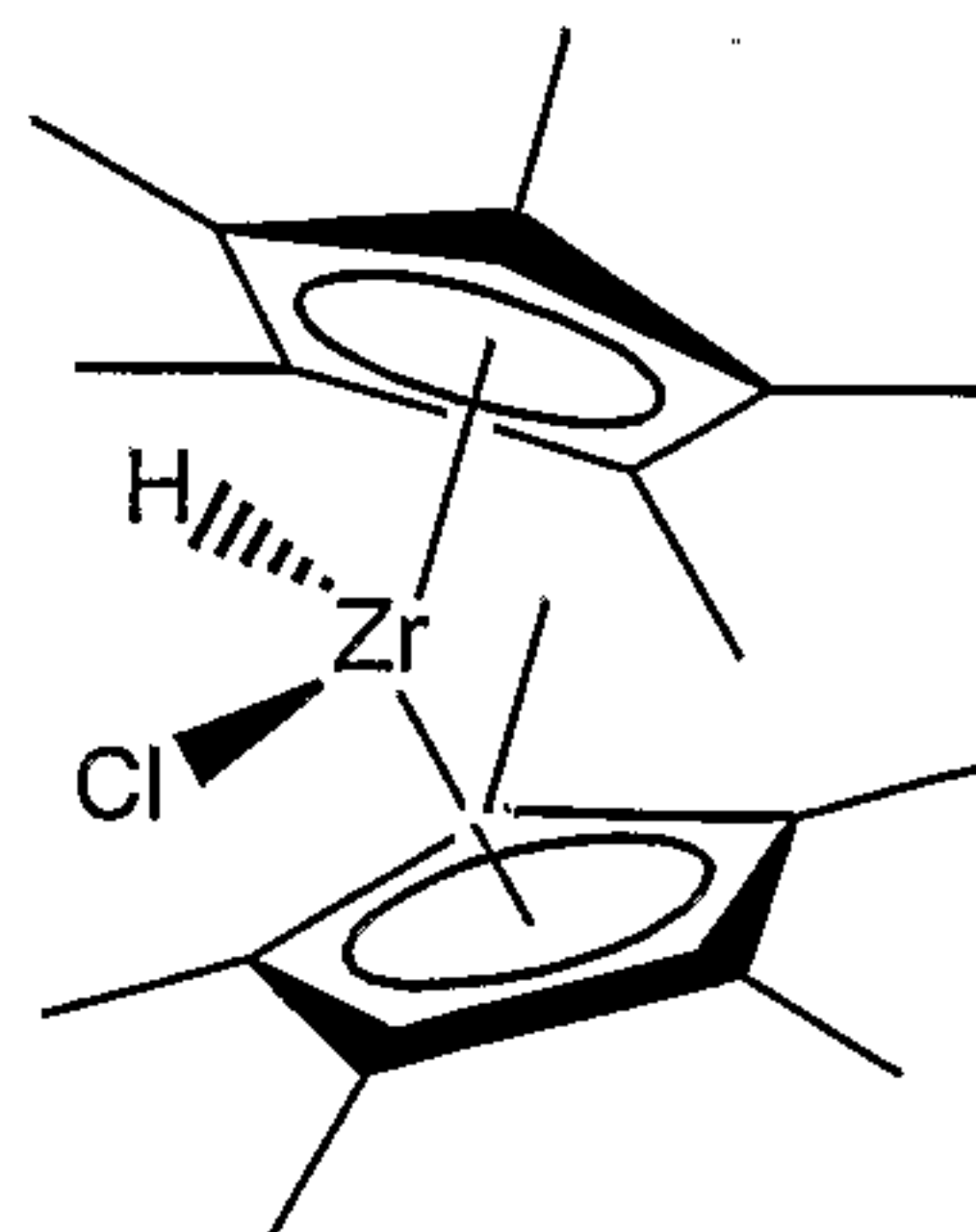
Bis(pentamethylcyclopentadienyl) zirconium chloride hydride
