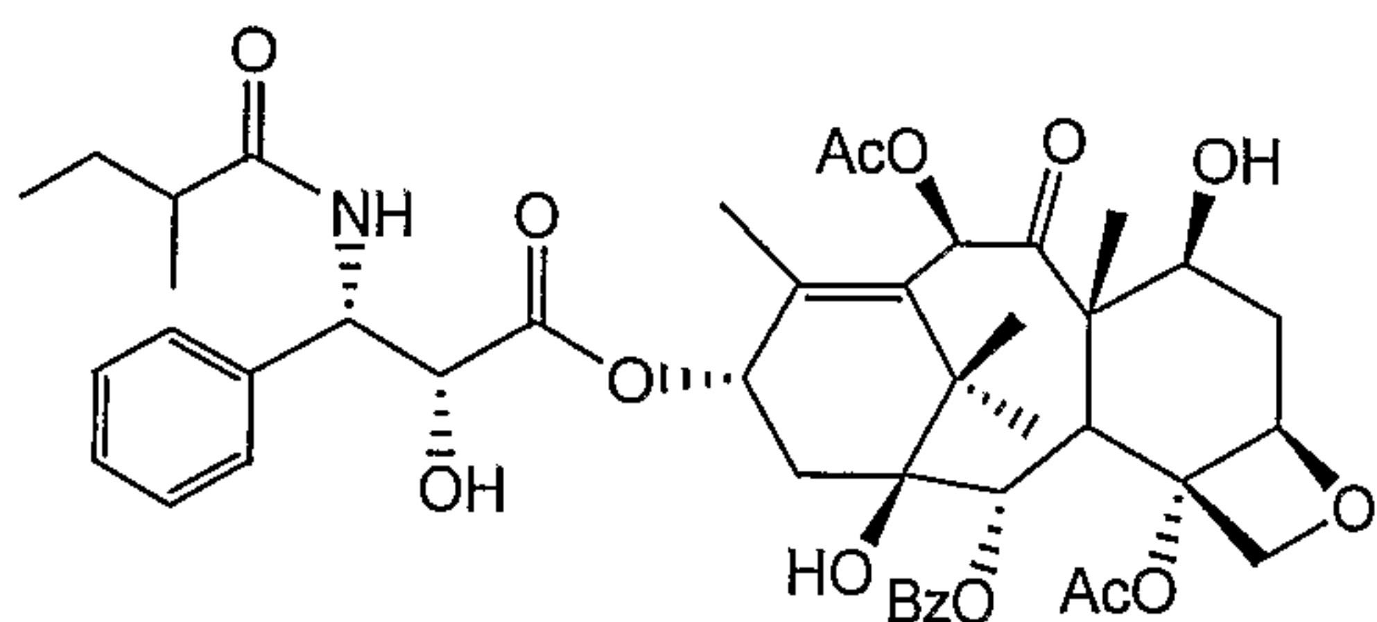
Taxol E
