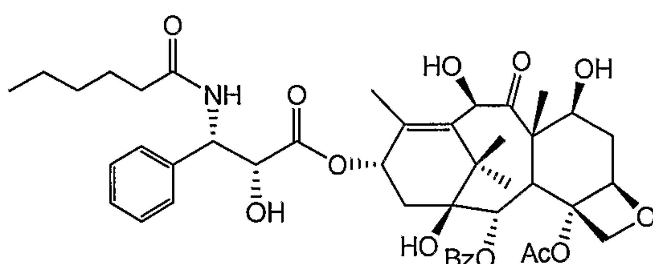
10-Deacetyltaxol C
