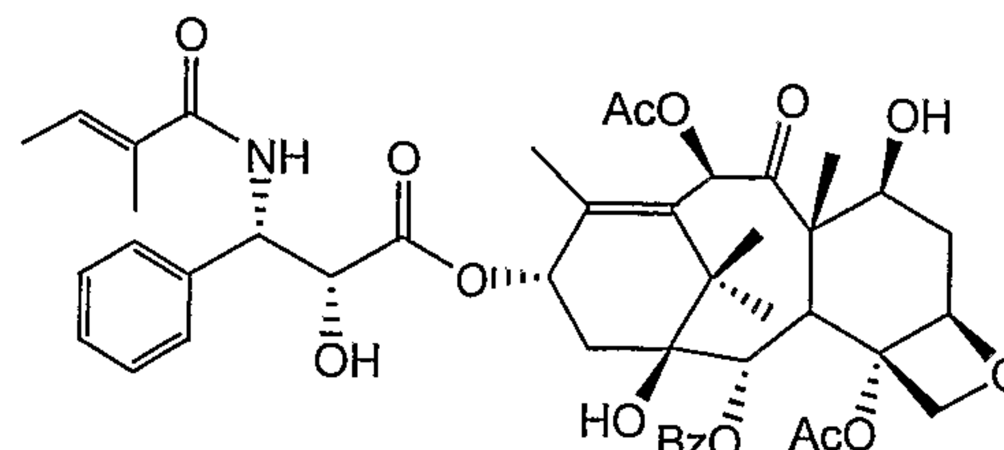
Taxol B (Cephalomannine)
