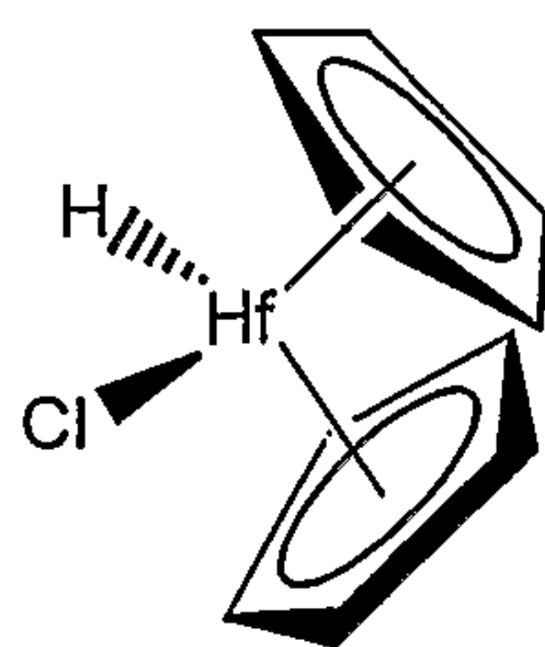
Bis(cyclopentadienyl) hafnium chloride hydride
