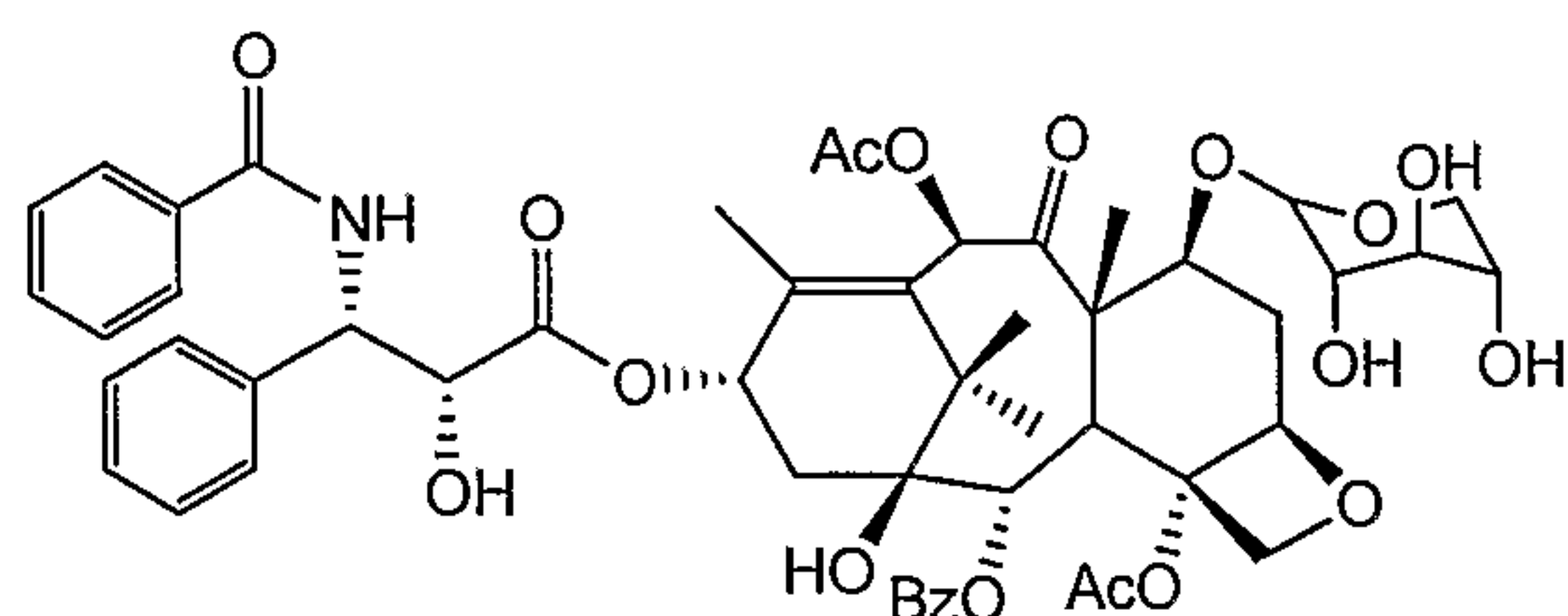
7-Xylosyltaxol A
