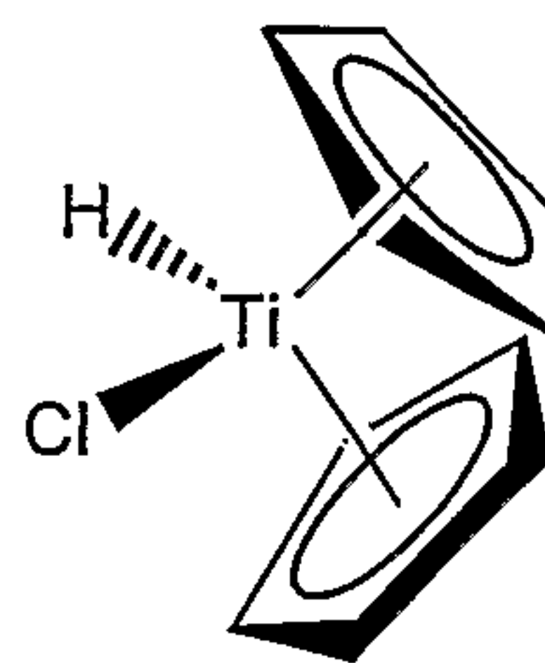
Bis(cyclopentadienyl) titanium chloride hydride
