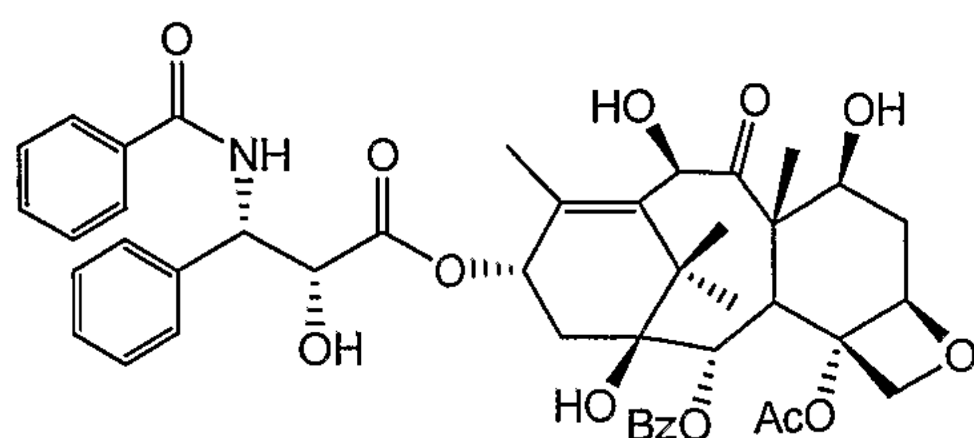
10-Deacetyltaxol A
