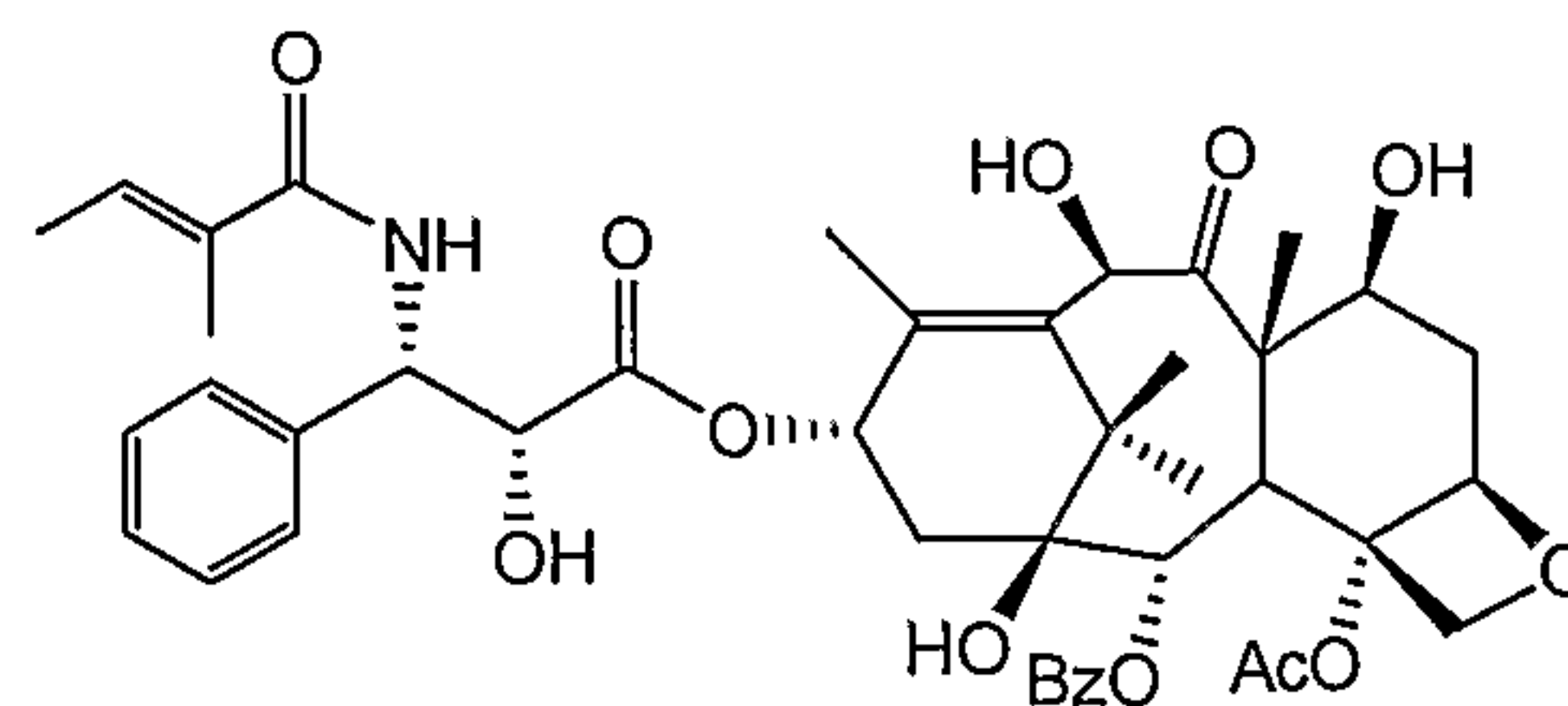
10-Deacetyltaxol B
