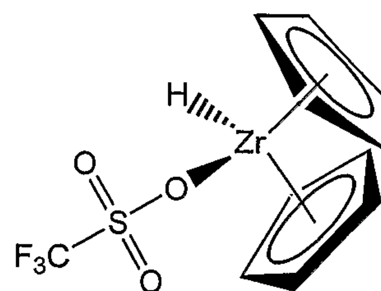
Bis(cyclopentadienyl) zirconium triflate hydride
