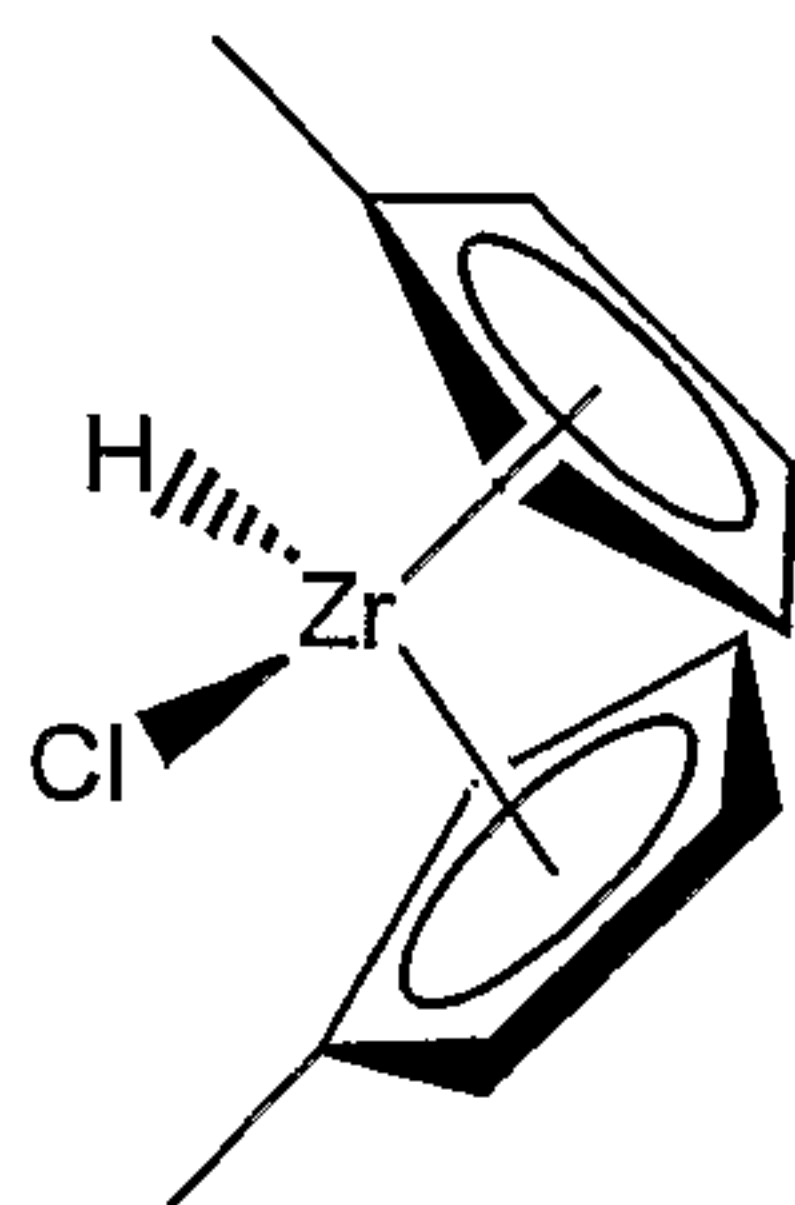
Bis(monomethylcyclopentadienyl) zirconium chloride hydride
