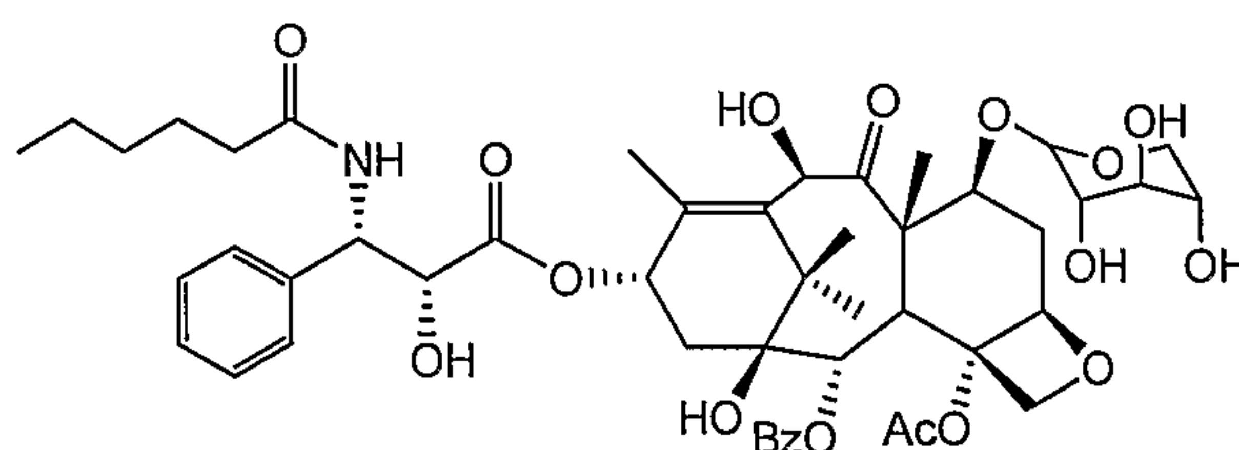
7-Xylosyl, 10-deacetyltaxol C
