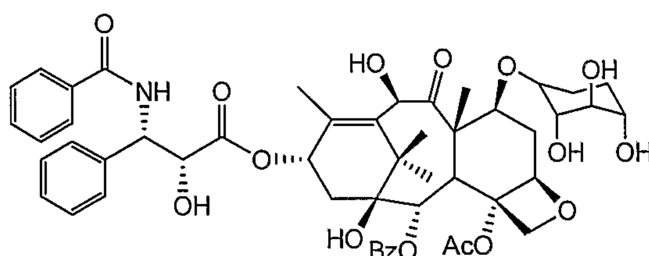
7-Xylosyl, 10-deacetyltaxol A
