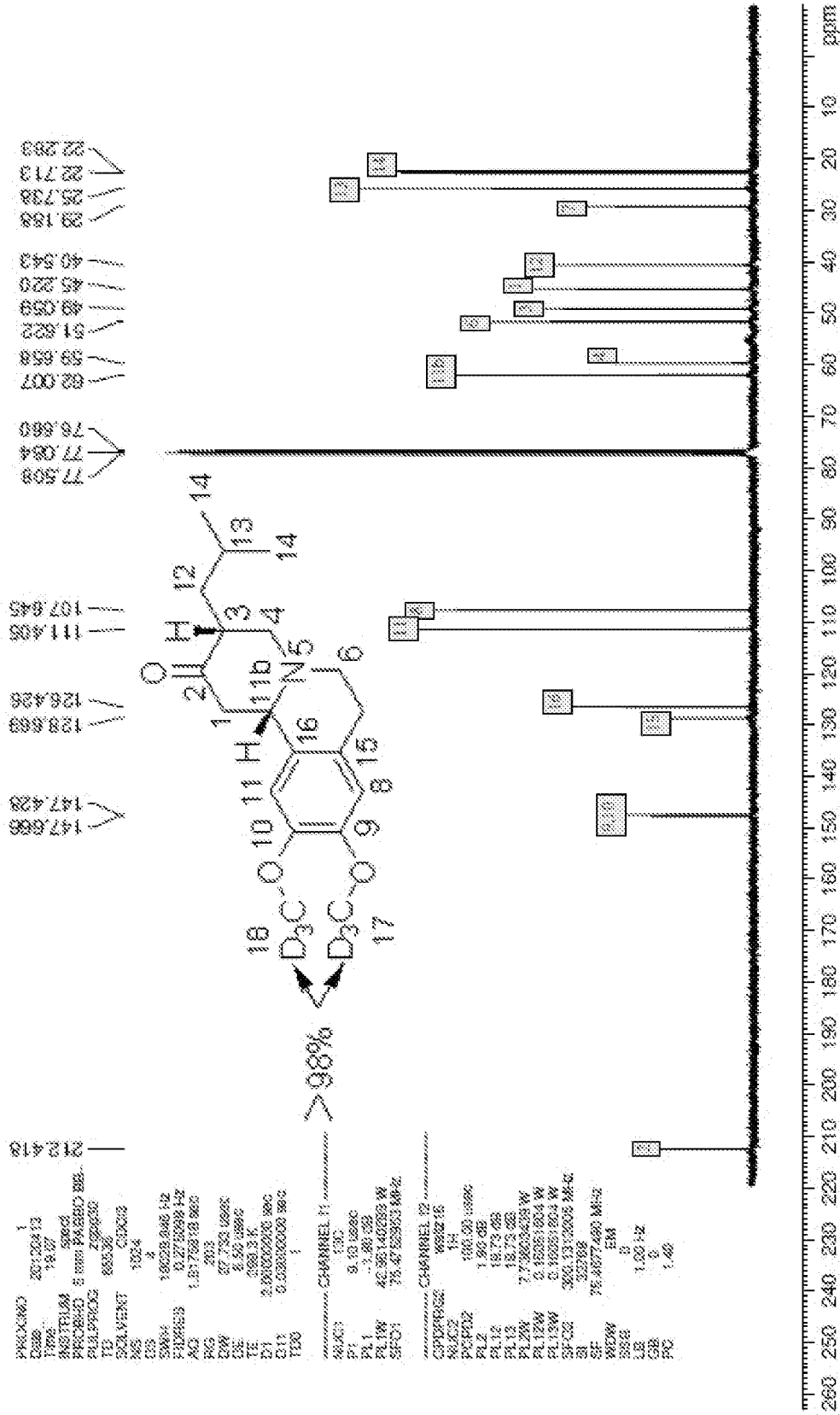
Figure 3: 13 C NMR of compound 1
