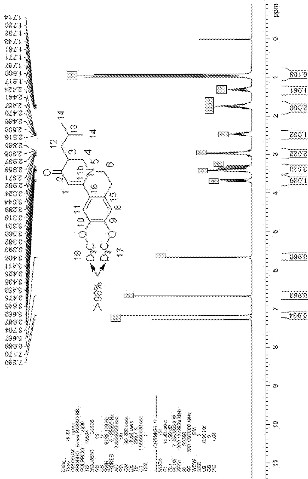
Figure 6: ^1\text{H} NMR of compound 2
