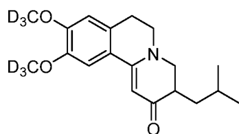
Compound 2
