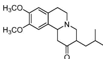
Tetrabenazine
