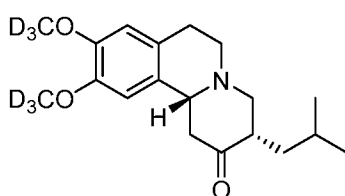
Compound 1 or
