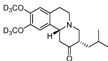
Compound 1
