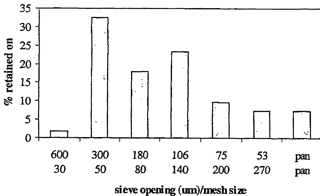
Particle Size Distribution of API, Lot N005B (sieve analysis)
