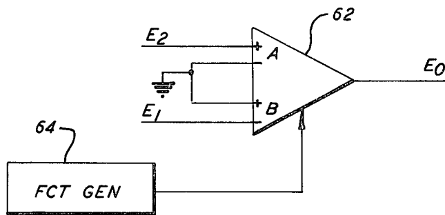
FIG. 4 Prior Art
