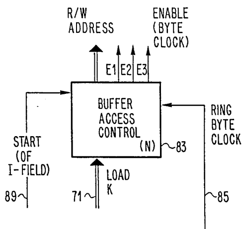
FIG. 6A BUFFER ACCESS CONTROL FOR VOICE PACKETS
