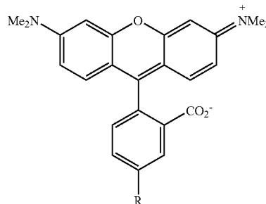
Tetramethylrhodamine
