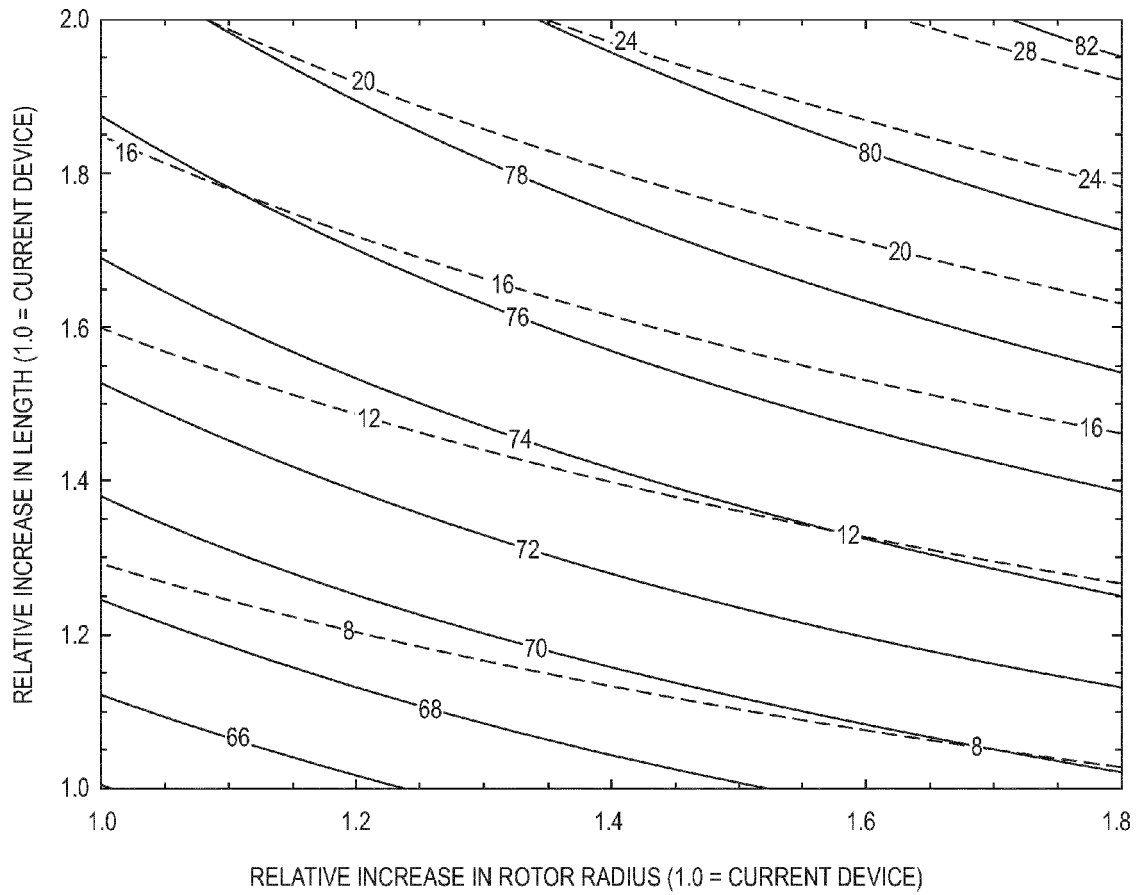
——— OUTLET HEMATOCRIT (%) - - - OUTLET PLASMA HEMOGLOBIN CONCENTRATION (mg/dL) (MEMBRANE TANGENTIAL VELOCITY CONSTANT) Fig. 4
