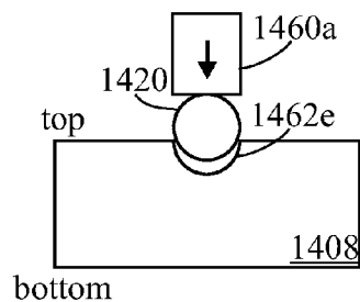
FIG. 14E Embedding a Wire in a Channel
