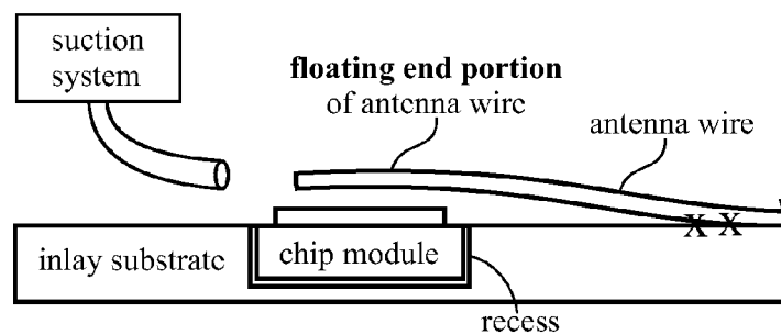
FIG. 16 Wire Straightening
