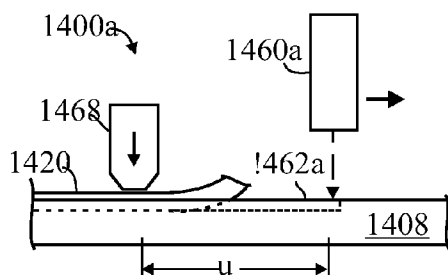
FIG. 14A Laser Ablation
