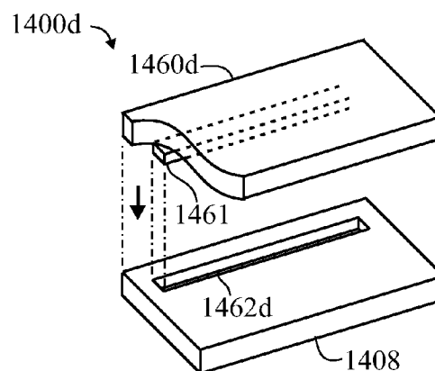
FIG. 14D Heat/Mold
