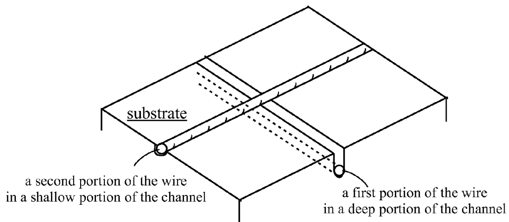
FIG. 15 Channel Crossings
