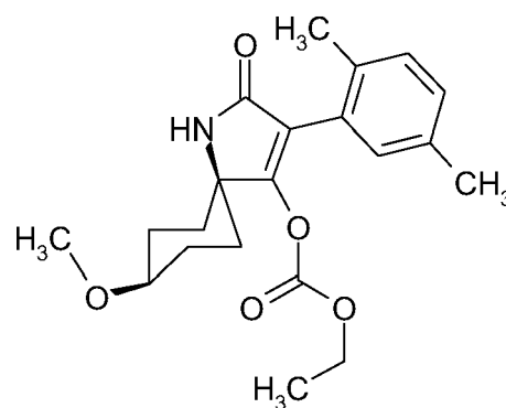
(I-2)
