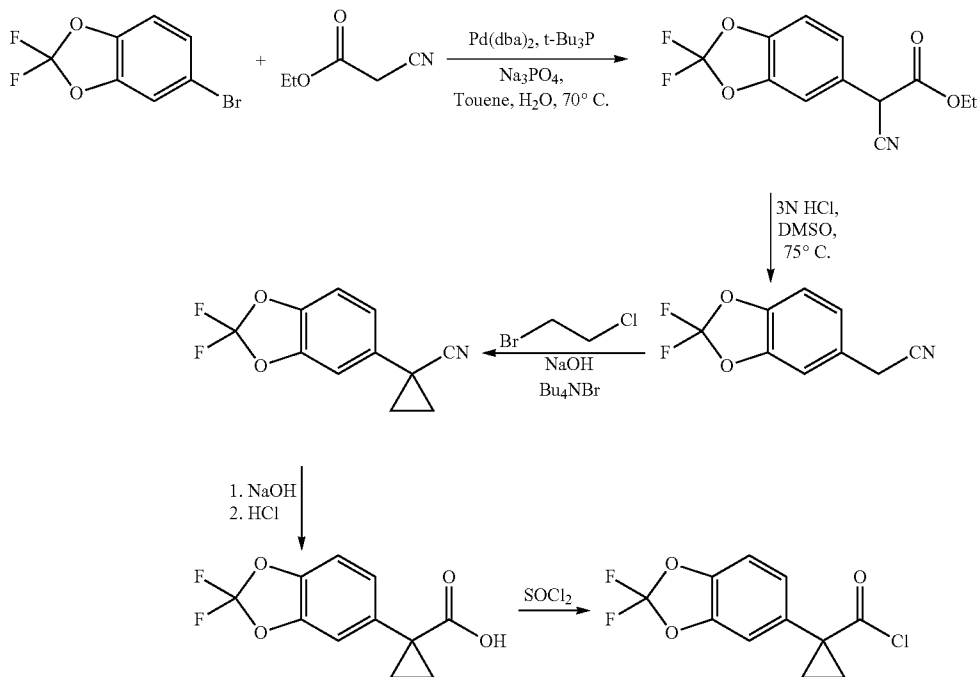
Scheme 2. Alternative synthesis of the requisite acid chloride.
