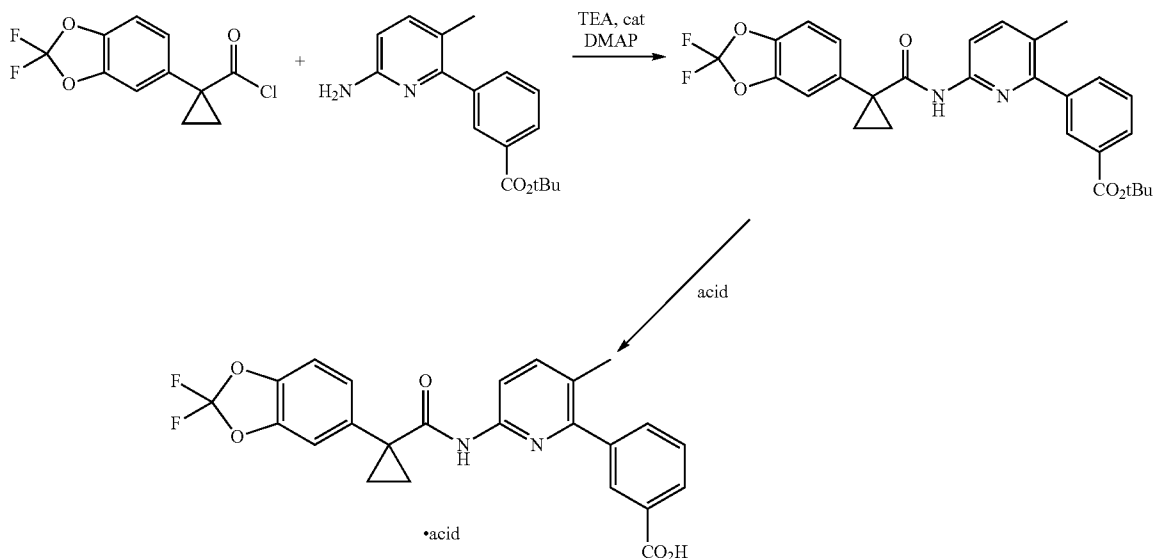
Scheme 4. Formation of an acid salt of Compound 1.
