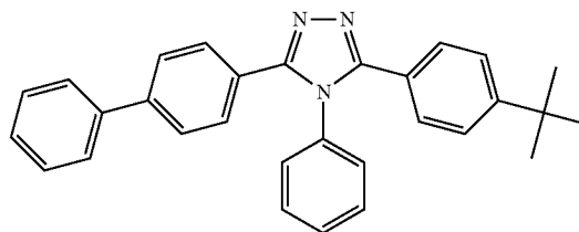
3-(4-Biphenyl)-4-phenyl-5-tert-butylphenyl-1,2,4-triazole C30H27N3
