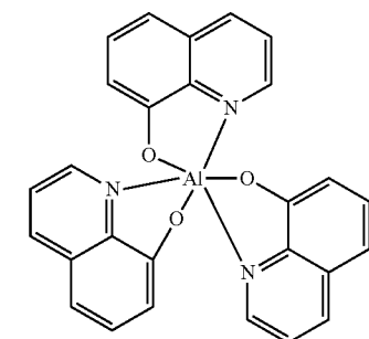
tris (8-hydroxy-quinolinato)-aluminium
