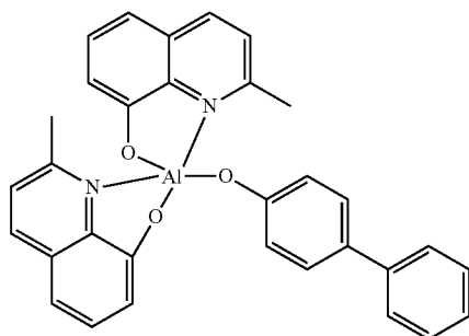
Bis-(2-methyl-8-quinolinolato)-4-(phenyl-phenolato)-aluminium-(III)
