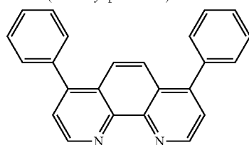
Bphen = bathophenanthroline (4,7-Diphenyl-1, 10-phenanthroline) C24H16N2
