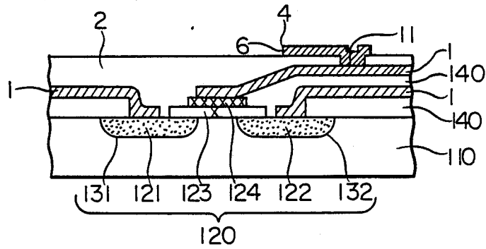
FIG. 6C PRIOR ART
