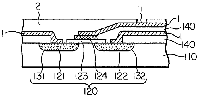
FIG. 5C PRIOR ART
