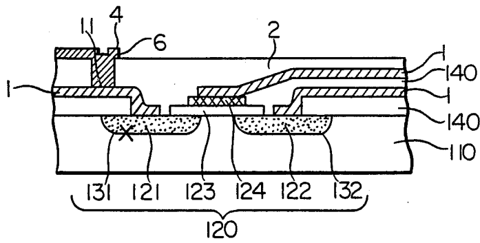
FIG. 6C PRIOR ART
