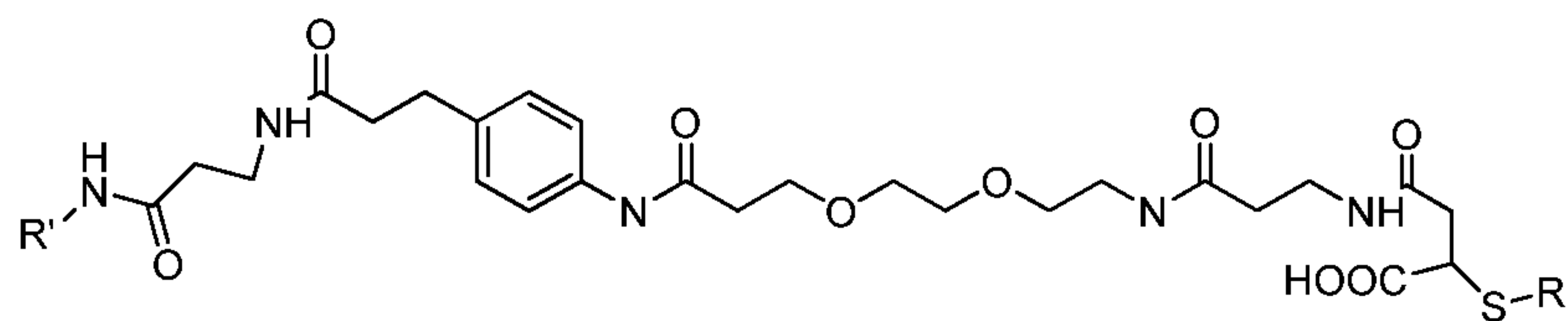
Scheme 1
