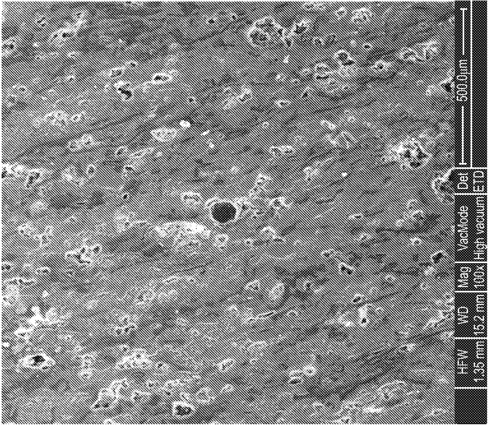
Magnification X 100 Air bubble size - 10 to 150 μm
