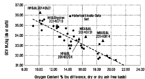
FIG. 1 Bio crude - Gross Calorific Value vs Oxygen Content
