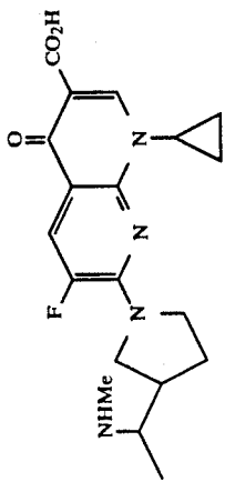
Enantiomer Mixture (Mixture B)
