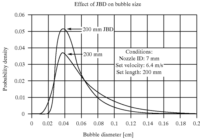
FIG. 1: pdf with and without JBD. Jet length = 200 mm, nozzle diameter = 7 mm, jet velocity = 6.4 m/s, JBD ID = 25 mm, JBD height = 50 mm, Frother 50 ppm Betafroth.
