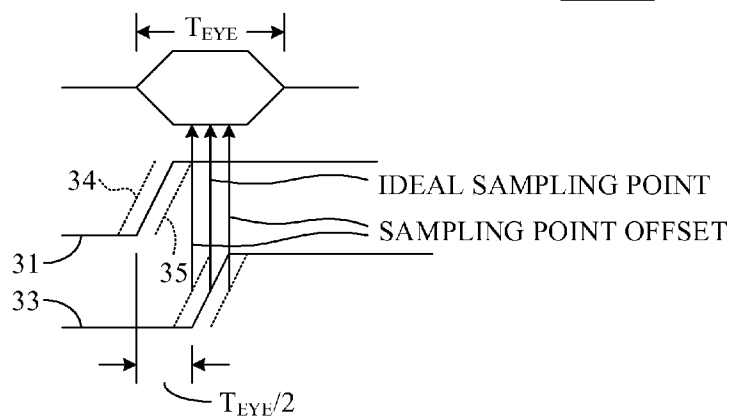
FIG. 2 (Prior Art)
