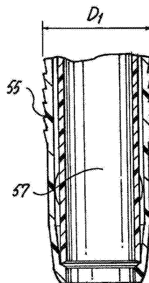
Fig. 10 (Prior Art)
