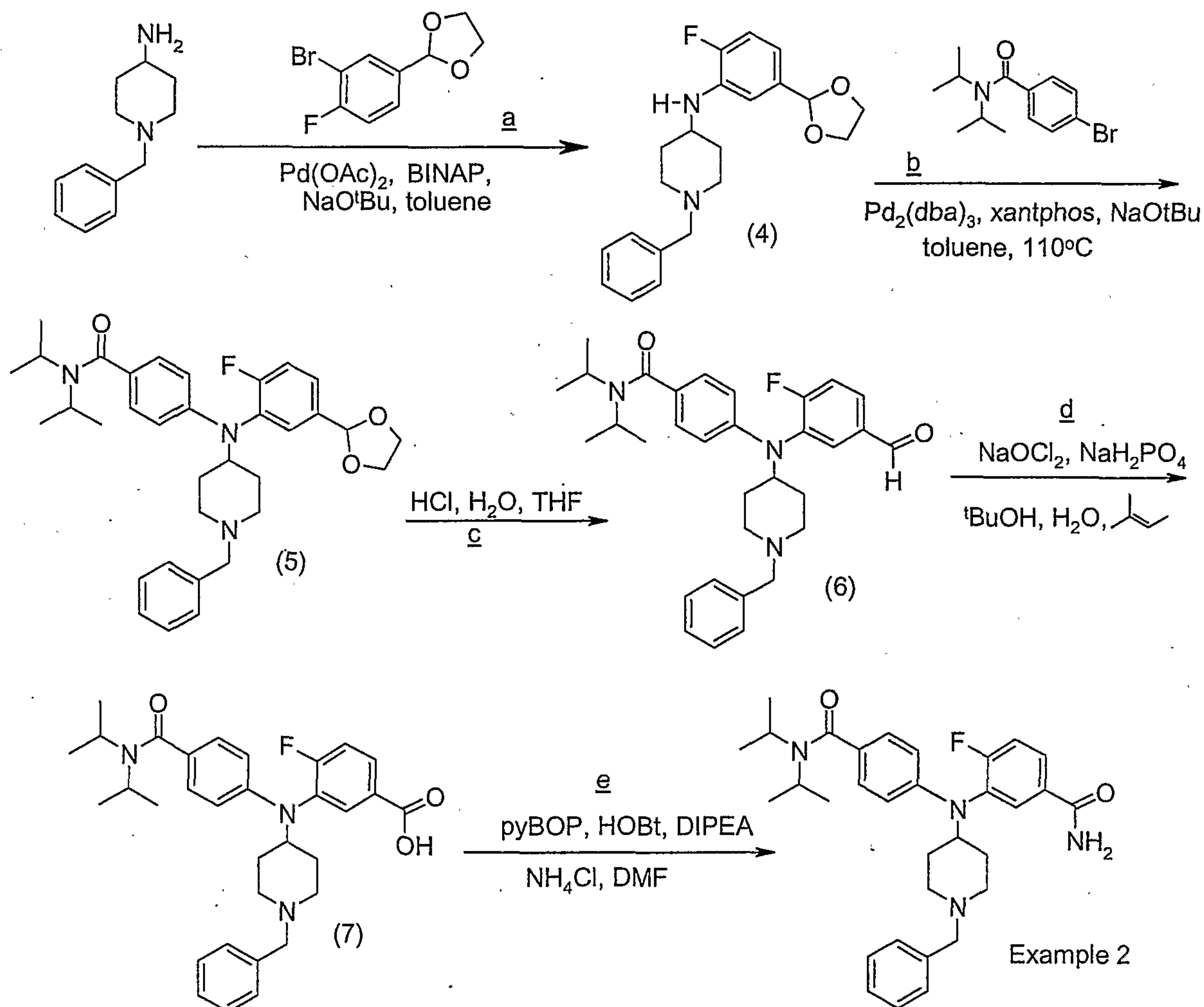
Scheme 2: Alternative synthesis Via Intermediate 7
