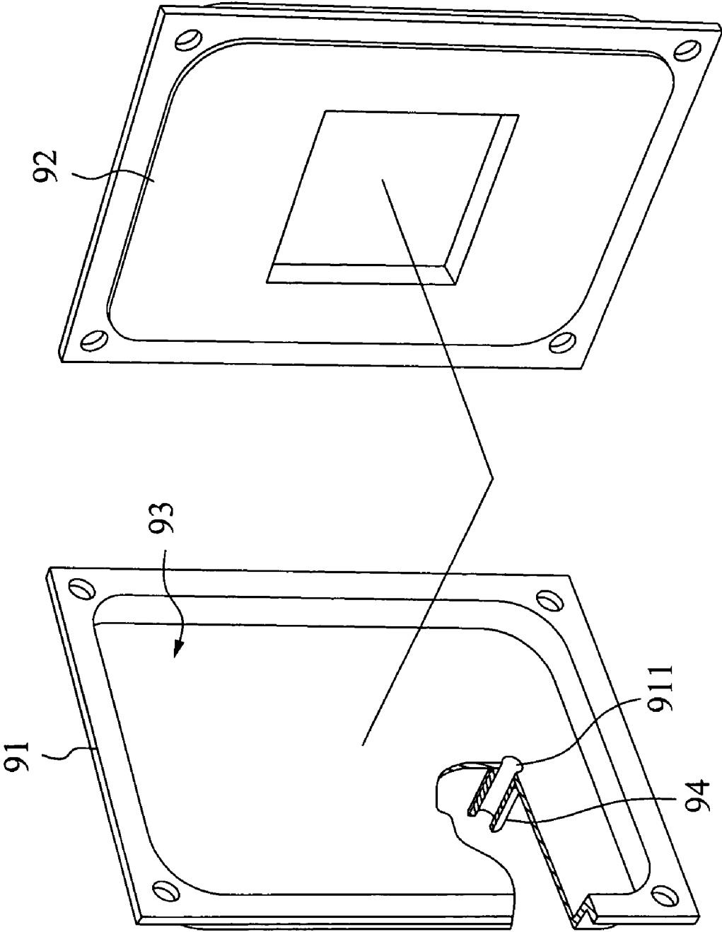
Fig. 1 (Prior Art)
