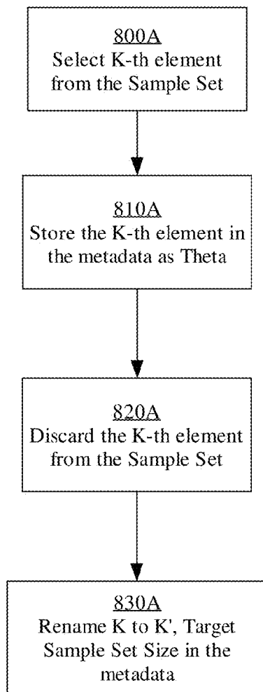
FIG. 8A - Fixed-Size to Theta Conversion
