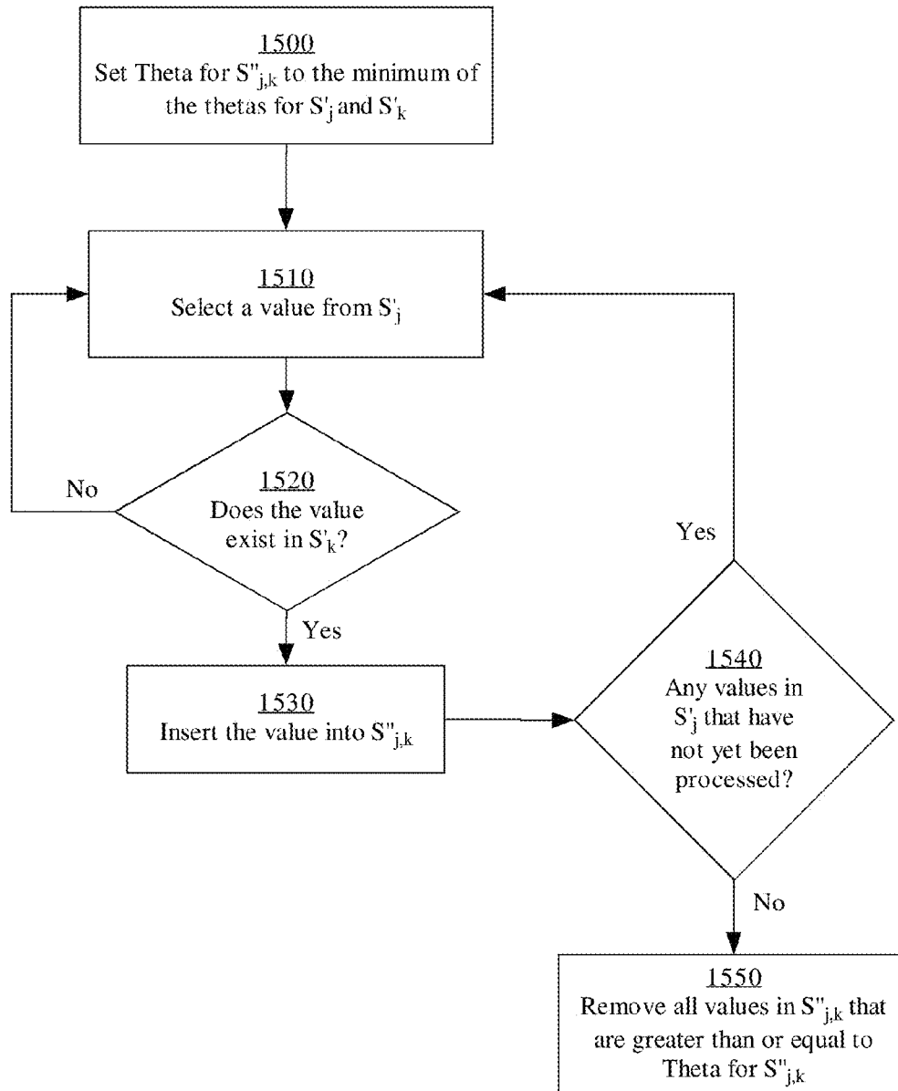
FIG. 15 - Intersection Operation on Theta Sketches
