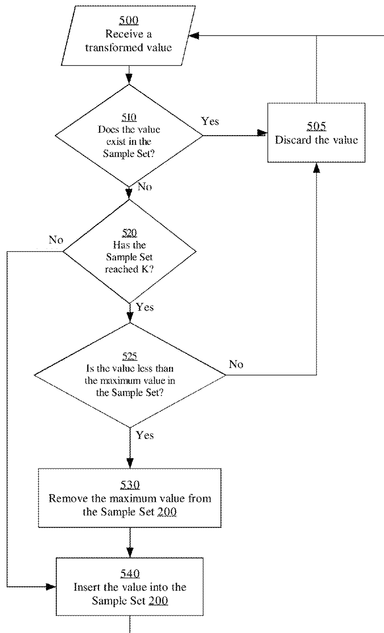
FIG. 5 - Fixed-Size Sketch Generation
