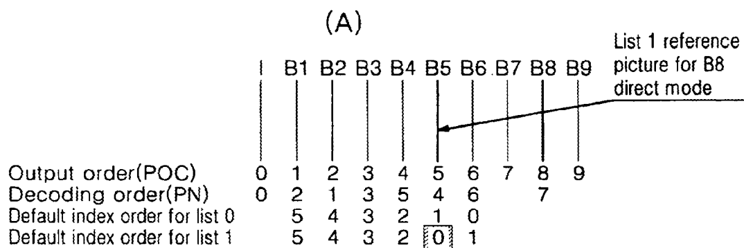
FIG. 2 (Related Art)
