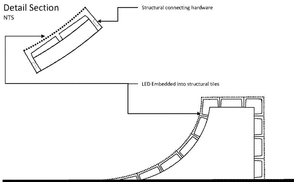
Video Ramp Assembly Type C – Section
