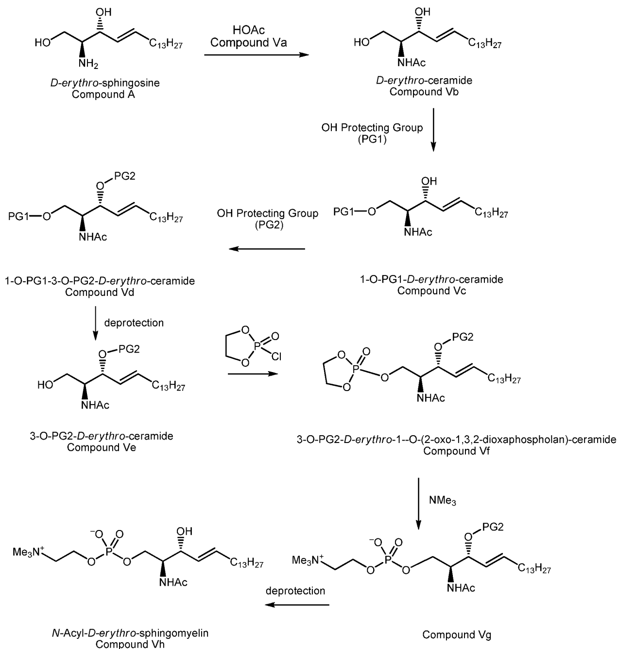
Scheme V
