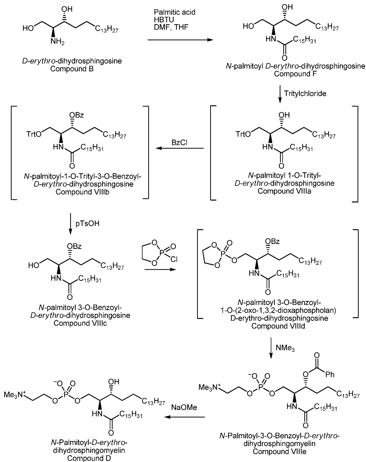
Scheme VIII
