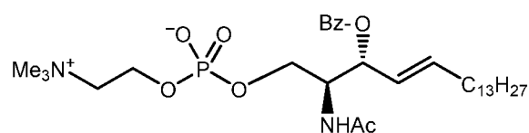
Compound VIIg ;
