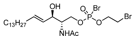
Compound XIIIb ;
