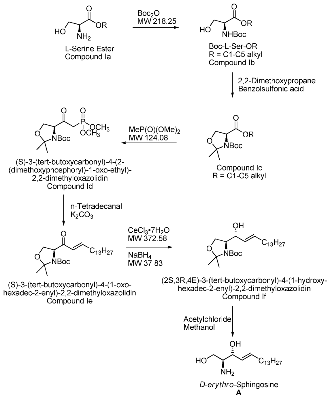
Scheme I
