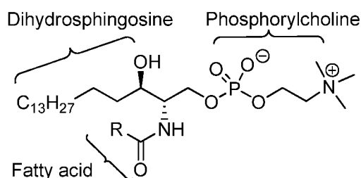
DIHYDROSPHINGOMYELINS
