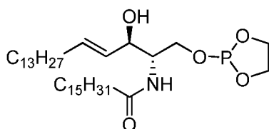
5 N-((2S,3R,E)-1-((1,3,2-dioxaphospholan-2-yl)oxy)-3-hydroxyoctadec-4-en-2-yl)palmitamide ;
