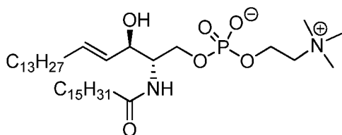
Compound C
