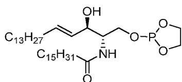
Compound XIVa
