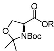
Compound Ic ;
