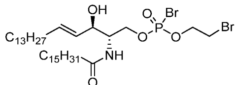
Compound XIVb
