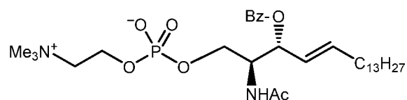
Compound VIIg
