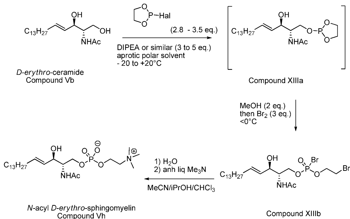
Scheme XIII
