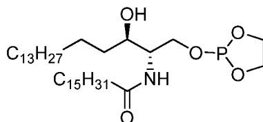
N-((2S,3R)-1-((1,3,2-dioxaphospholan-2-yl)oxy)-3-hydroxyoctadecan-2-yl)palmitamide
