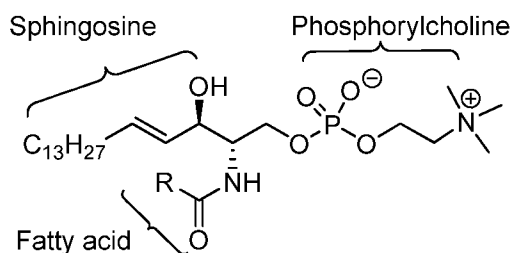
SPHINGOMYELINS
