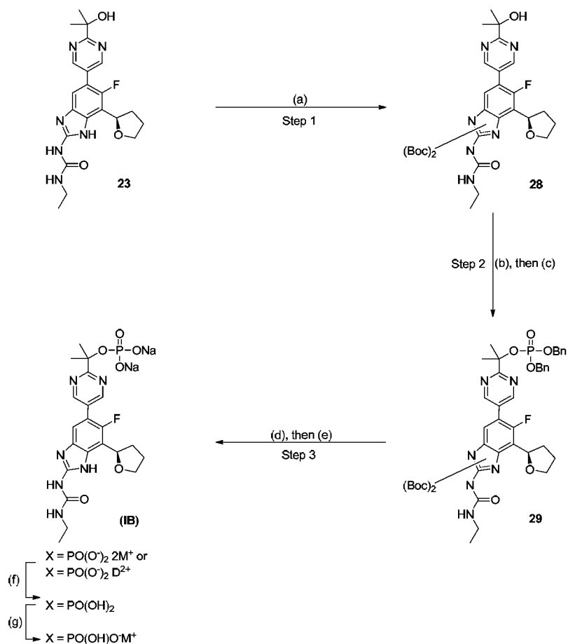
[00203] Scheme 3
