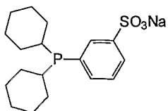
Ligand A
