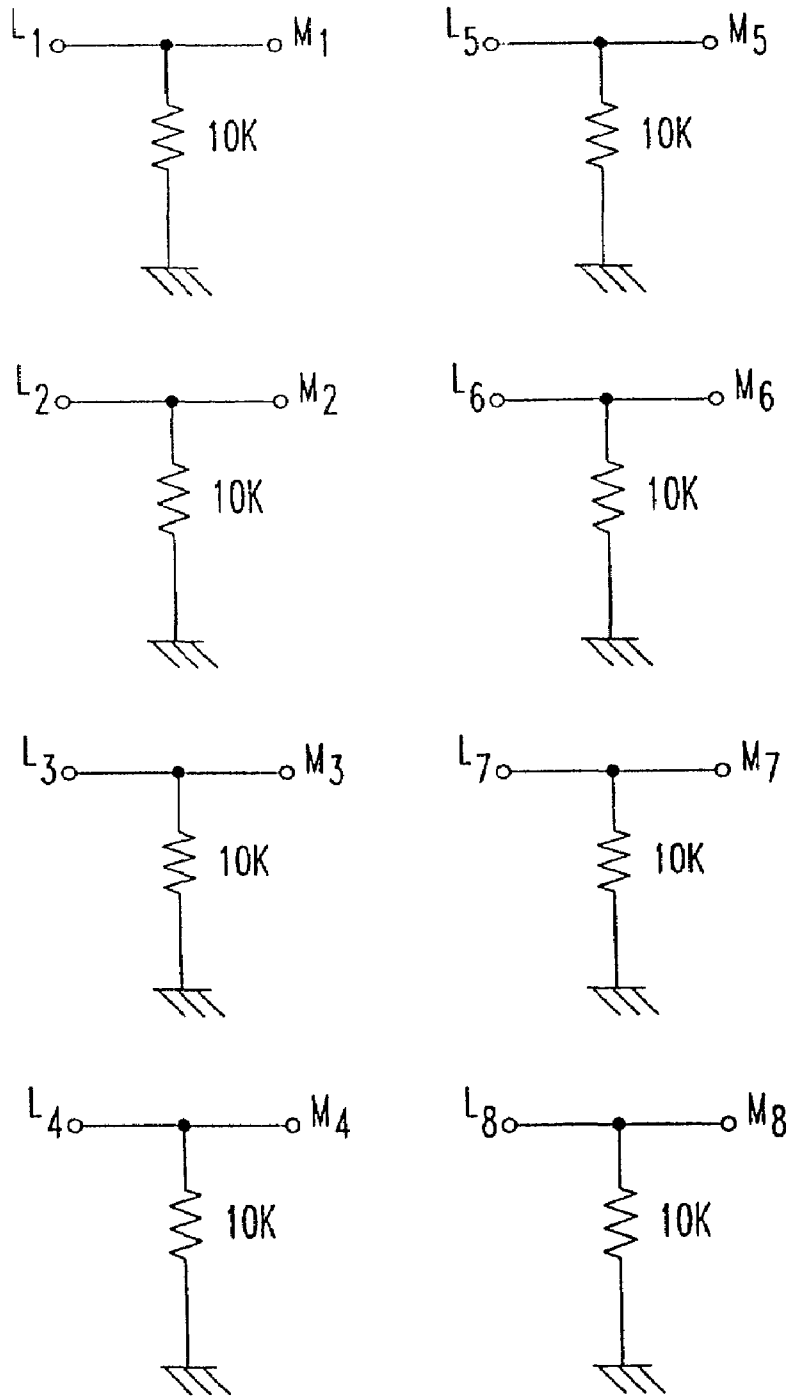
OUTPUT MUX LOAD RESISTORS
