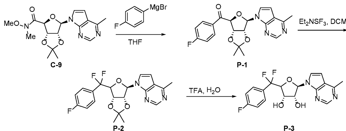
Scheme P
