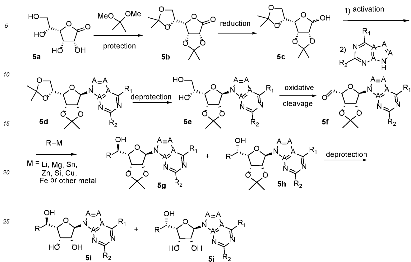
Scheme 5:
