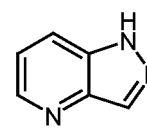
pyrazolo[4,3-d]pyridine (pyrazolo[4,3-d]pyridinyl)
