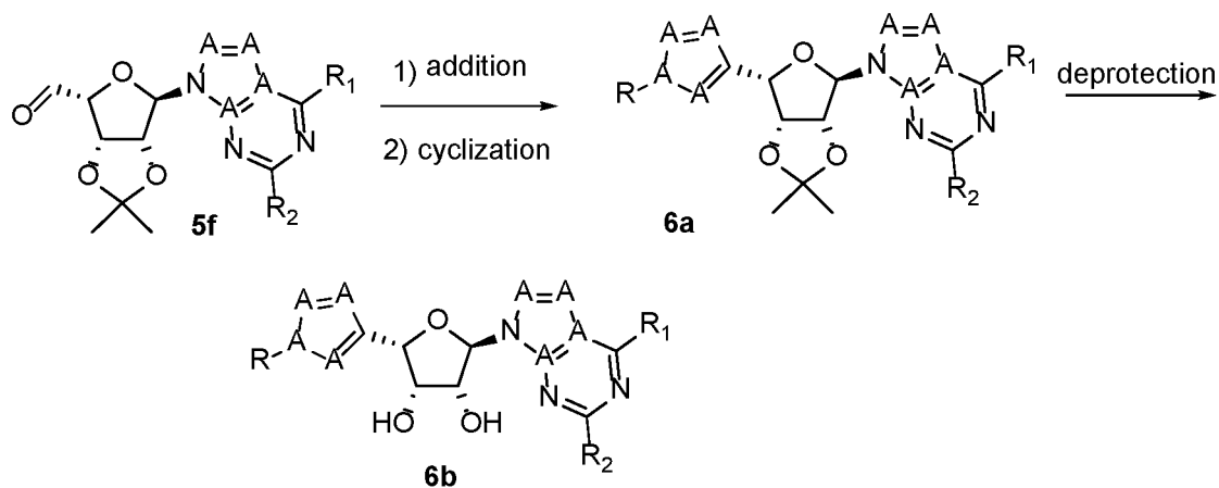
Scheme 6:
