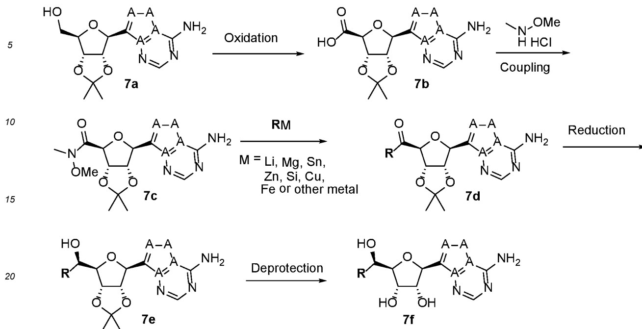
Scheme 7:
