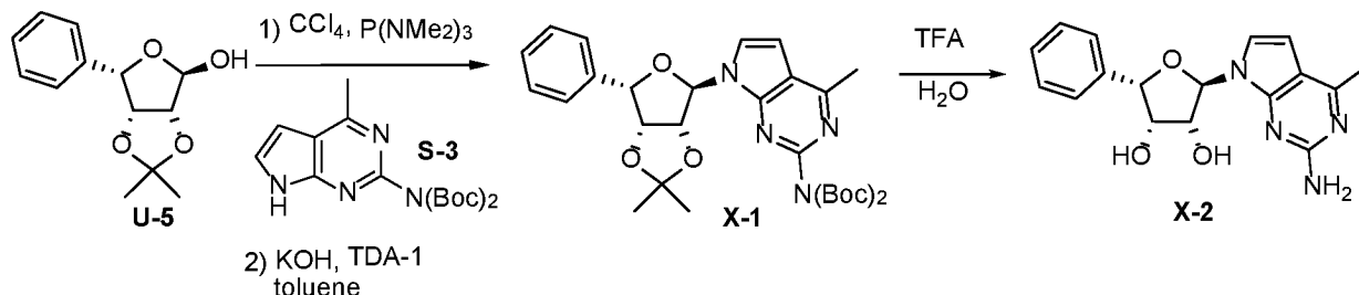
Scheme X
