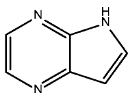
5H-pyrrolo[3,2-b]pyrazine
