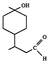
FIG. 4 is the NMR spectrum for the peak indicated by reference numeral "13" of the GLC profile of FIG. 1 containing the compounds having the structures:
