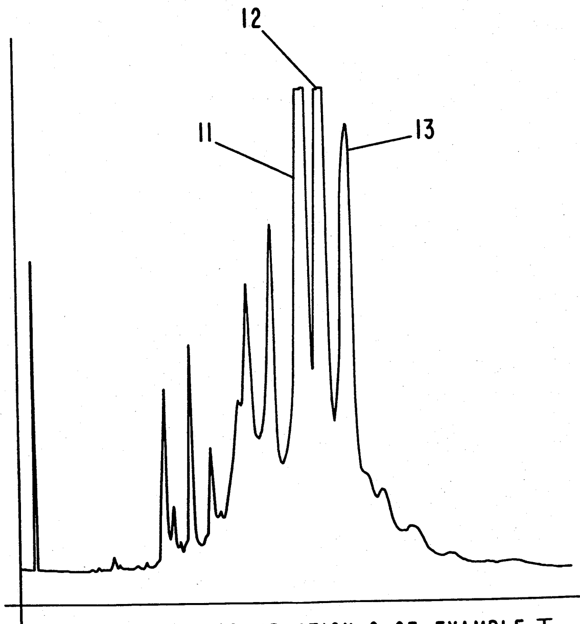
GLC PROFILE FOR FRACTION 6 OF EXAMPLE I.
