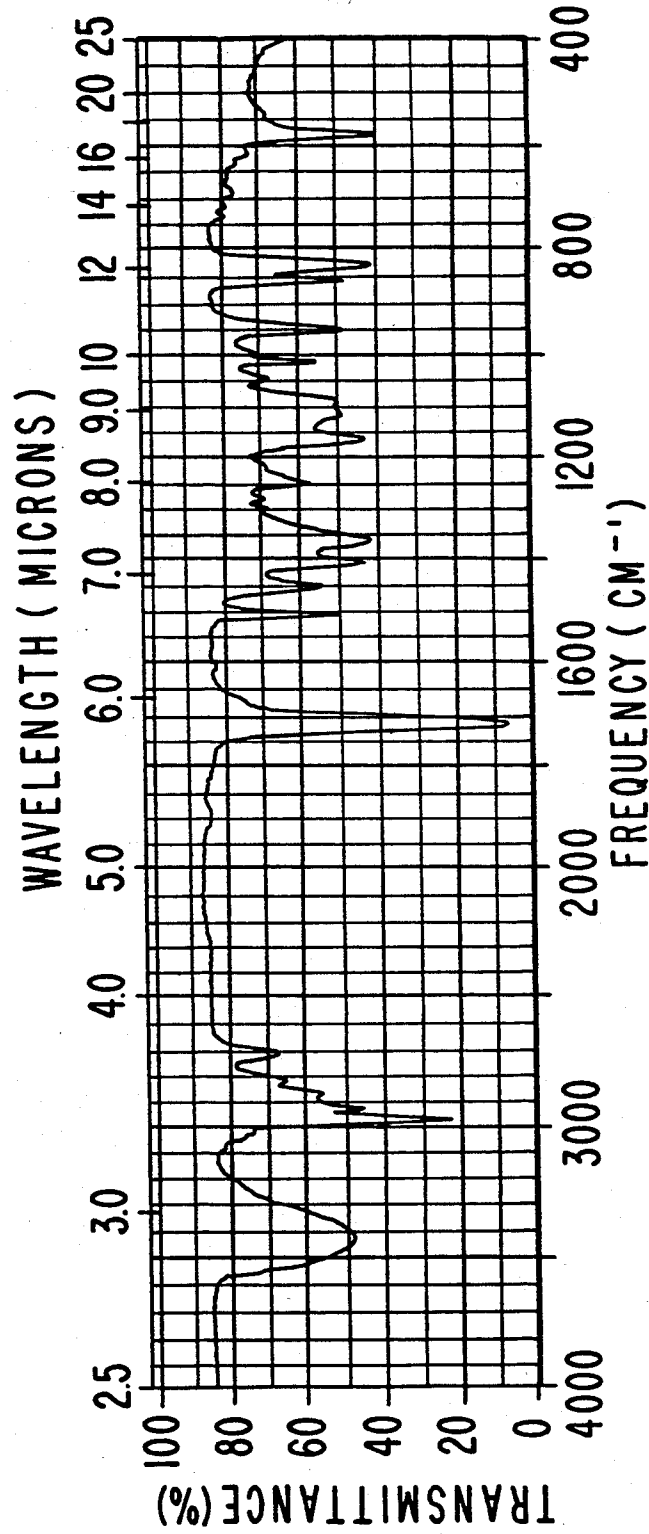
IR SPECTRUM FOR FRACTION 6 OF EXAMPLE III. FIRST DISTILLATION
