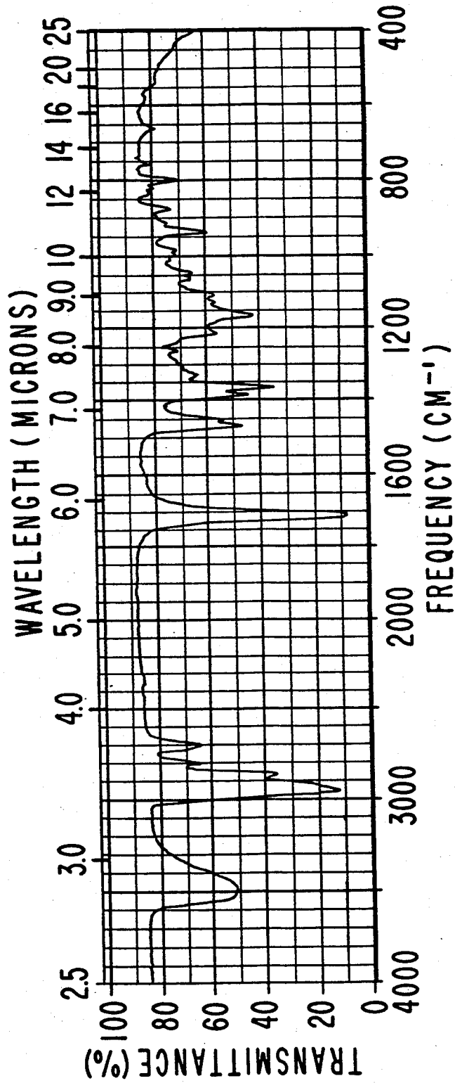
IR SPECTRUM FOR EXAMPLE II.
