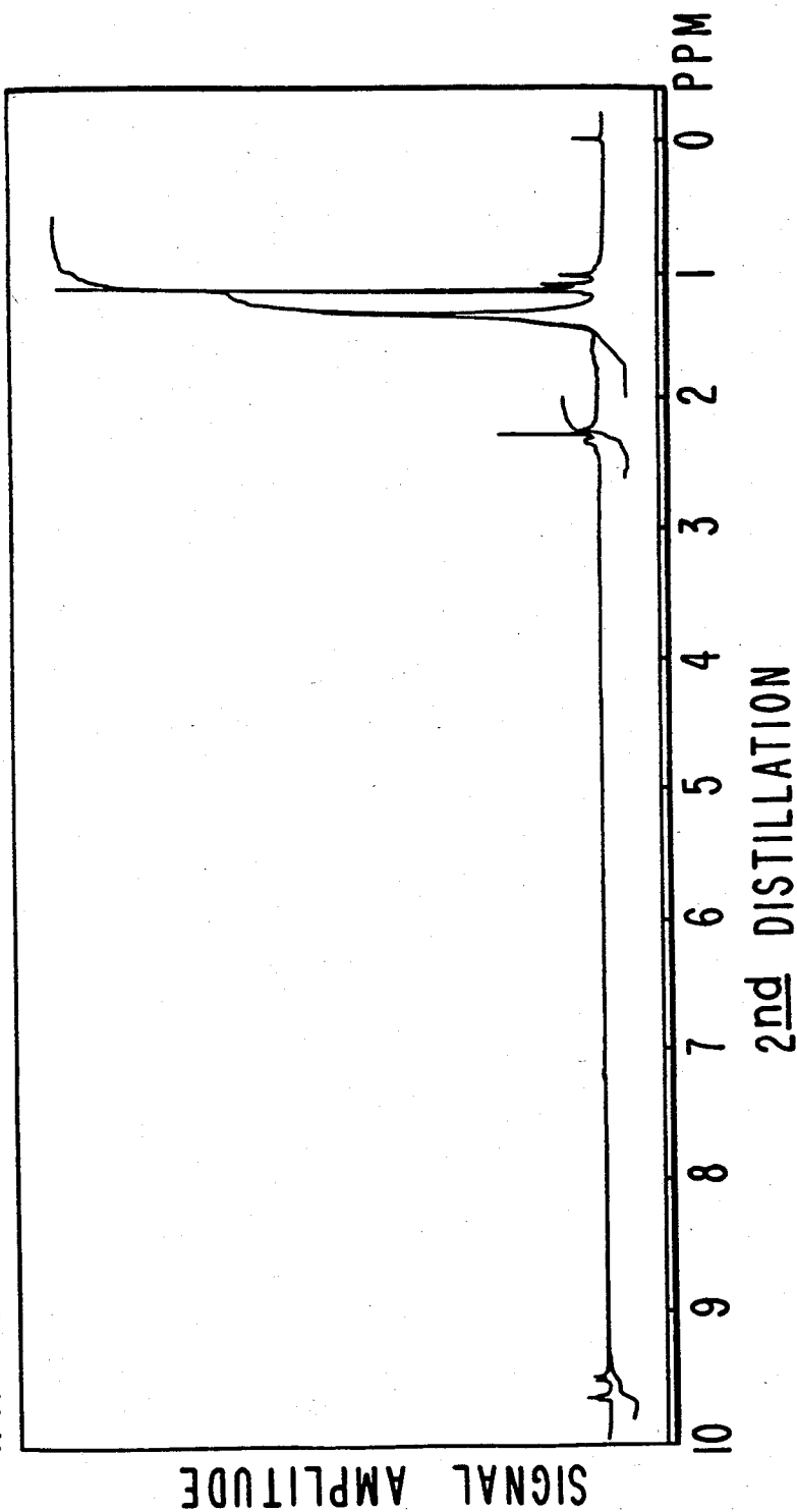
NMR SPECTRUM FOR FRACTION 4 OF EXAMPLE IV.
